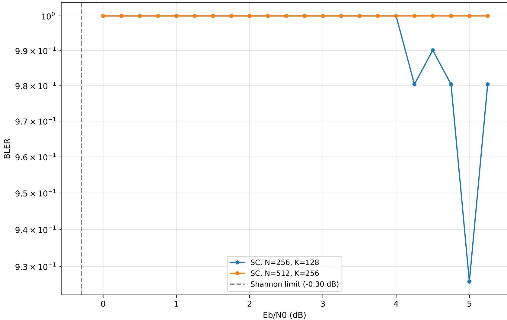
SC Decoder BLER
