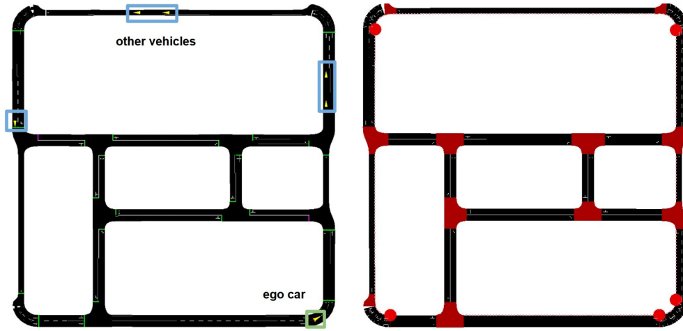
Fig. 6. CARLA-SUMO co-simulation: the SUMO GUI for traffic visualization (left) and NetEdit for network and work-zone lane configuration (right).
