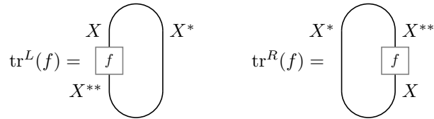
FIGURE 17.3.1. Left and right traces; pivotal isomorphism \delta_X and its inverse are not shown.
