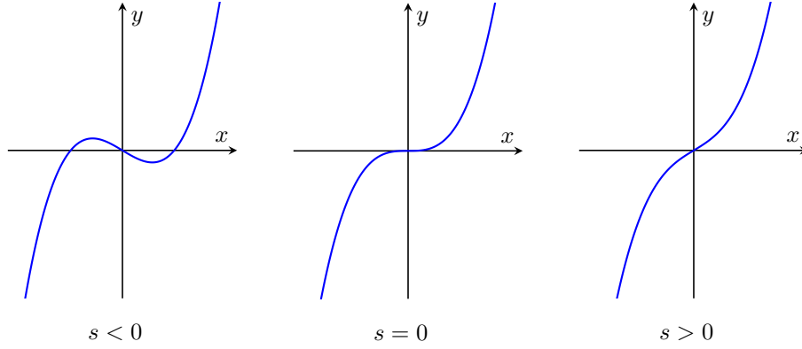
FIGURE 4.2.1. Birth-death of critical points in the family f_s = x^3 + sx .
