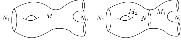
FIGURE 1.3.1. Cutting a manifold M into two manifolds M_1 and M_2 along a codimension-one submanifold N . The gluing axiom asserts that Z_M = Z_{M_2} \circ Z_{M_1} .
