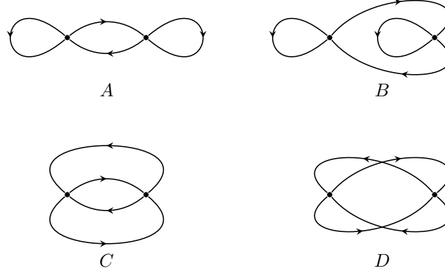
FIGURE 4.3.1. Possible shapes of the critical level set S . Note that for the last graph, intersection points are not vertices.
