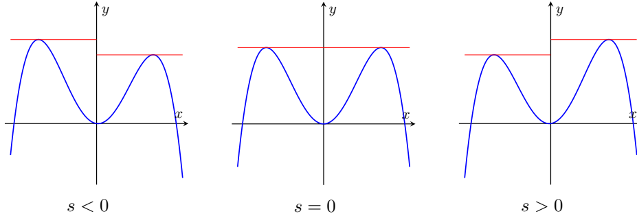
FIGURE 4.2.2. Crossing of critical values in the family f_s = 2x^2 - x^4 + sx .
