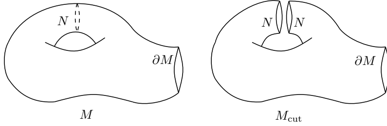
FIGURE 3.3.1. Cutting a manifold M along a codimension-one submanifold N .
