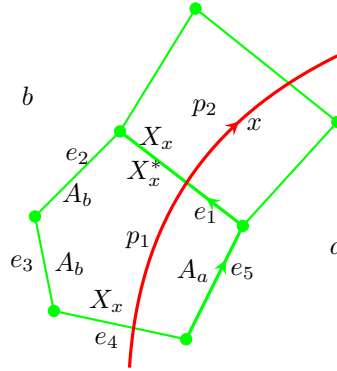
FIGURE 13.2.1. Example of vector spaces assigned to the edges of 2-cell p_1 . Regions to the left and right of defect x are labelled by algebras b and a respectively.
