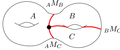
FIGURE 13.1.1. A stratified manifold decorated with algebras A , B and C on different regions. Defects are shown in red, and are labelled by bimodules. Defects require a choice of orientation, which is suppressed here for brevity.
