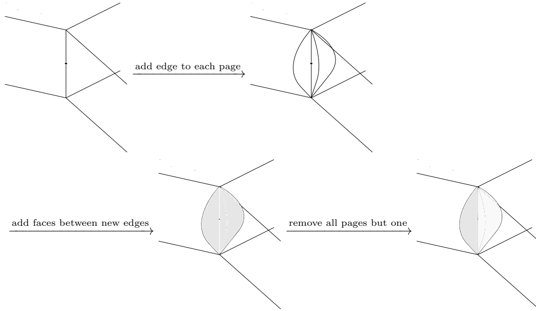
FIGURE 19.4.4. Decomposing an open book into a single page book
