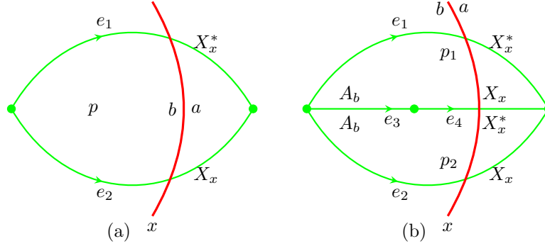
FIGURE 13.3.1. Example(I) of a local modification of cell decomposition used in Lemma 13.3.1
