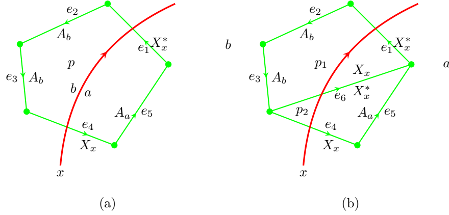
FIGURE 13.3.2. Example(II) of a local modification of cell decomposition used in Lemma 13.3.1
