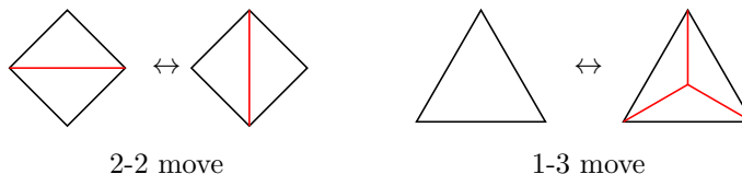
FIGURE 11.2.1. Pachner moves in dimension 2
