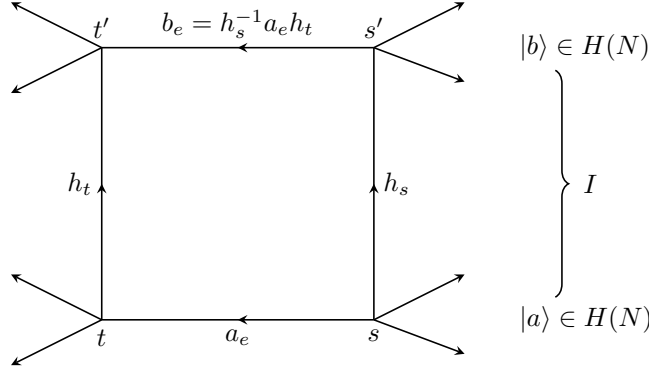
FIGURE 19.6.1. A sample configuration appearing in the \sum_{l_{\text{flat}}} Z(N \times I, l_{\text{flat}}) . Bottom of the diagram shows a portion of configuration |a\rangle assigned to a closed 2-manifold N . |a\rangle assigns an a_e \in G to each edge e , but we are showing only the edge e between s and t here. We label the vertical edges by elements h_v of G^{v(N)} for each v \in v(N) . The flatness condition imposes that the configuration |b\rangle on the other end of interval I is a gauge transformation of |a\rangle , i.e. |b\rangle = |h.a\rangle .
