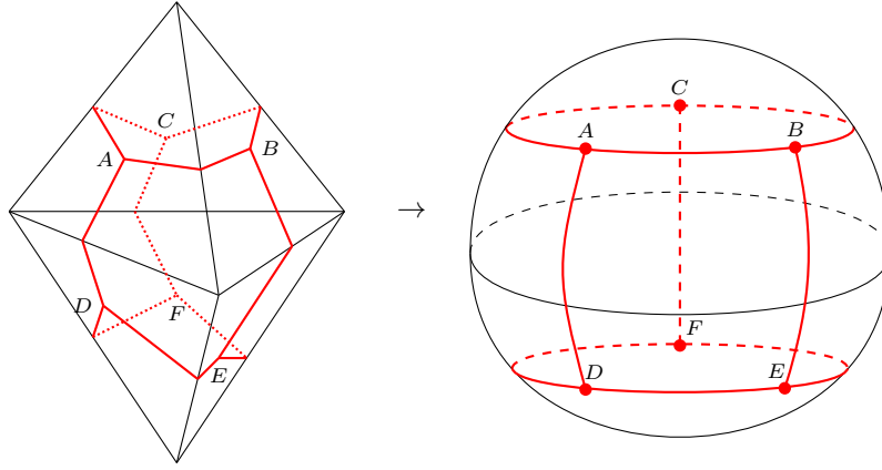
FIGURE 19.3.1. The dual graph on the boundary of a 3-cell
