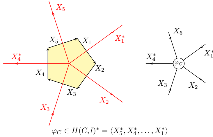
FIGURE 19.3.2. Coloring of the dual graph
