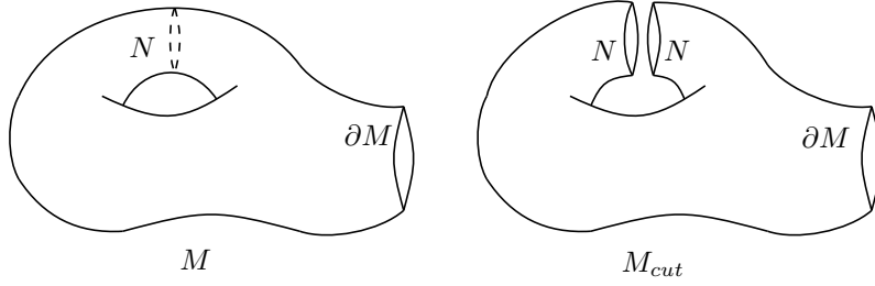
FIGURE 3.3.1. Cutting of a manifold M along a codimension one submanifold N
