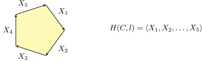
FIGURE 19.2.1. Defining the state space for a 2-cell
