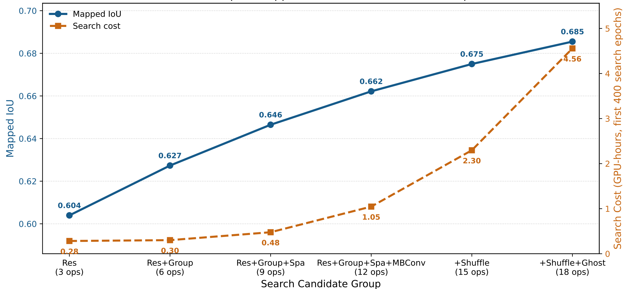
Candidate Group vs Mapped IoU and Search Cost (400 epochs)
