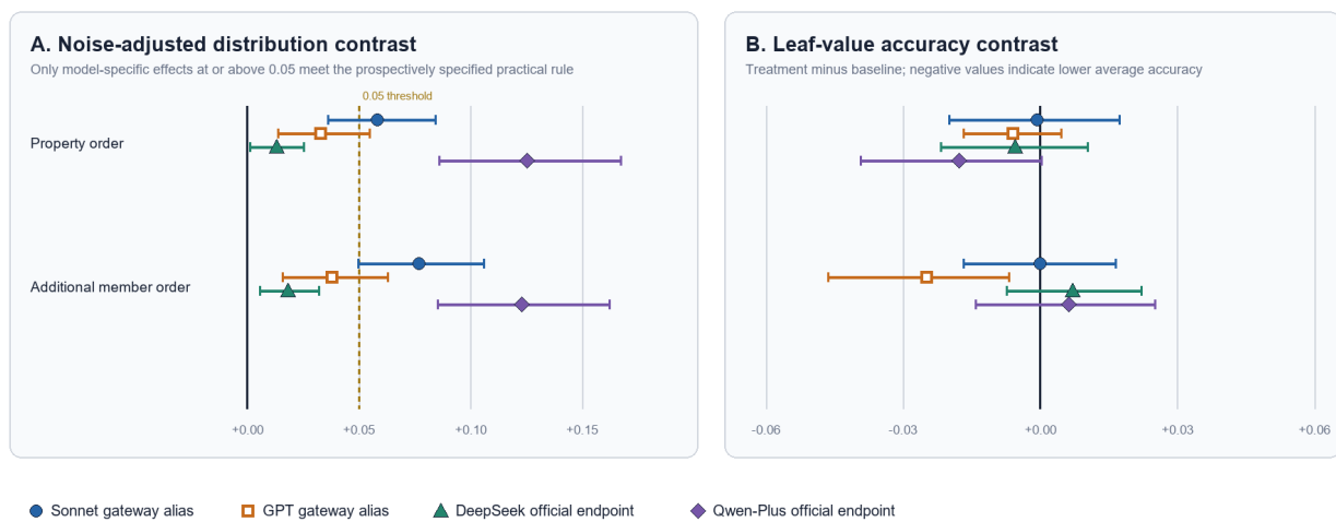
Fig. 3 Decomposed order effects across the four core text-mode deployments; the supplemental endpoint panel is tabulated in Table 3.
