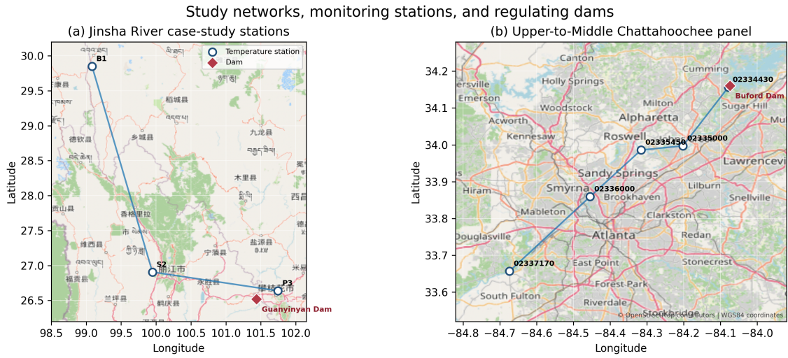
498 499 Figure 1. Study networks, monitoring stations, and regulating dams.. (a) Jinsha River case- 500 study stations and Guanyinyan Dam. B1, S2, and P3 are separated by 463 and 558 river km; 501 straight connecting segments indicate station order rather than the detailed river centerline. (b) 502 Upper-to-Middle Chattahoochee sites from immediately below Buford Dam through the Atlanta 503 reach. Station coordinates are documented inventory locations. The Guanyinyan symbol uses a 504 cartographic RCC-dam coordinate; the scientific distance context is the official 27 river km to P3. 505 Basemap © OpenStreetMap contributors.
