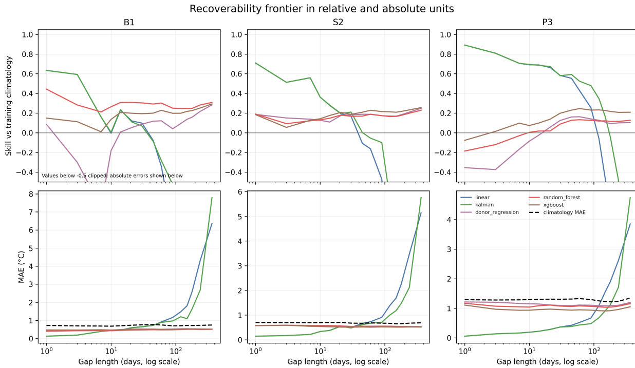
525 526 Figure 4. Recoverability in relative and absolute units.. Top: climatology-relative skill for five 527 representative stable methods. Values below -0.5 are clipped for readability. Bottom: the same 528 methods' MAE in degrees C, with paired training-climatology MAE shown as a black dashed line. 529 All methods use common artificial cells.
