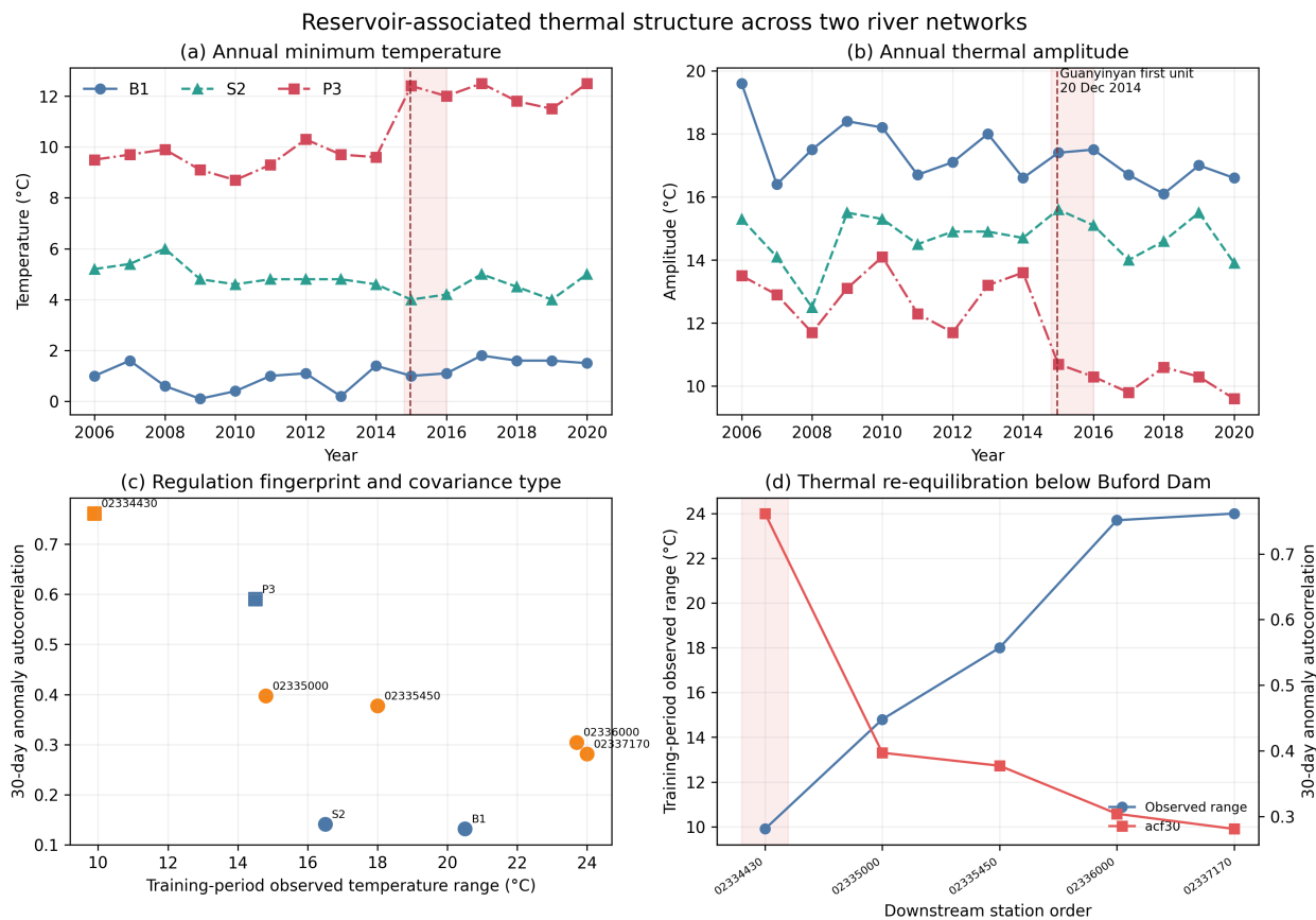
508 Figure 2. Reservoir-associated thermal structure across two networks.. (a) Annual minimum 509 stream temperature and (b) annual amplitude at B1, S2, and P3; the dashed line marks first-unit 510 generation at Guanyinyan on 20 December 2014 and shading covers commissioning. The line is 511 engineering context, not an estimated change date; formal method-sensitive results are in Figure 512 S1. (c) Fitting-period temperature range versus lag-30 anomaly autocorrelation. Squares are 513 memory-dominated and circles donor-dominated. (d) Chattahoochee downstream profile. Range 514 increases and memory decreases away from Buford Dam. These are observational associations, 515 not a causal heat-budget attribution.
