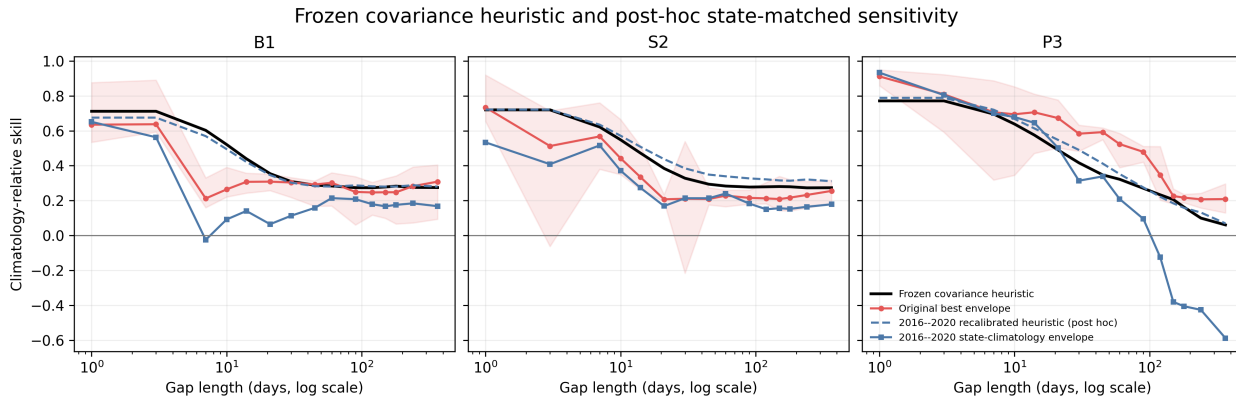
517 518 Figure 3. Frozen covariance heuristic and post-hoc thermal-state control.. Best-roster-envelope 519 climatology-relative skill and the train-only heuristic at B1, S2, and P3. Red/black use the original 520 2006-2015 calibration and denominator; blue re-scores fixed predictions and recalibrates the 521 heuristic to 2016-2020. The blue analysis overlaps evaluated years and diagnoses nonstation- 522 arity; it is not predictive evidence. Shading is the 95% anchor/year bootstrap interval for the 523 original descriptive envelope.
