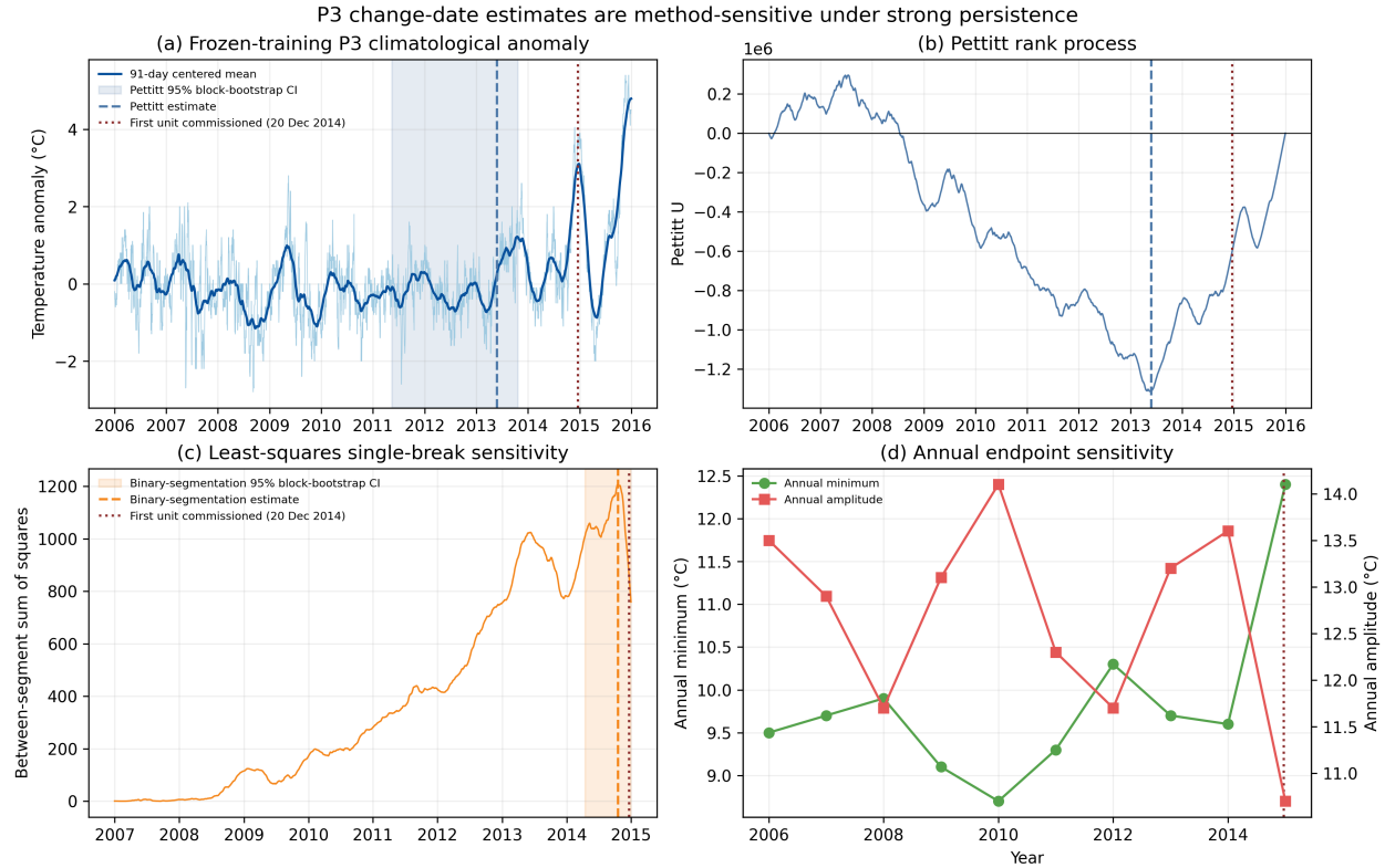
Figure 1: P3 change-date sensitivity
