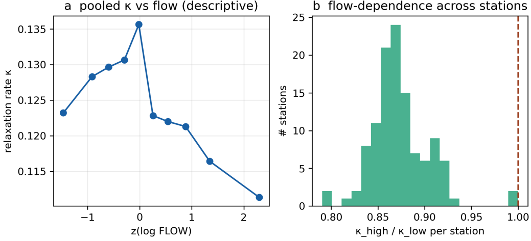
Figure 7. Dynamic relaxation rate \kappa on the 120-station USGS panel. (a) \kappa binned by standardised log-flow (pooled); (b) per-station ratio \kappa(\text{high flow})/\kappa(\text{low flow}) . The flow dependence seen on the three reservoir stations does not generalise — \kappa rises with flow at 0 % of stations on the 120-station panel (and 24 % on the 40-station pilot), median ratio 0.87 — so we retract the flow-dependent thermal-memory claim.
