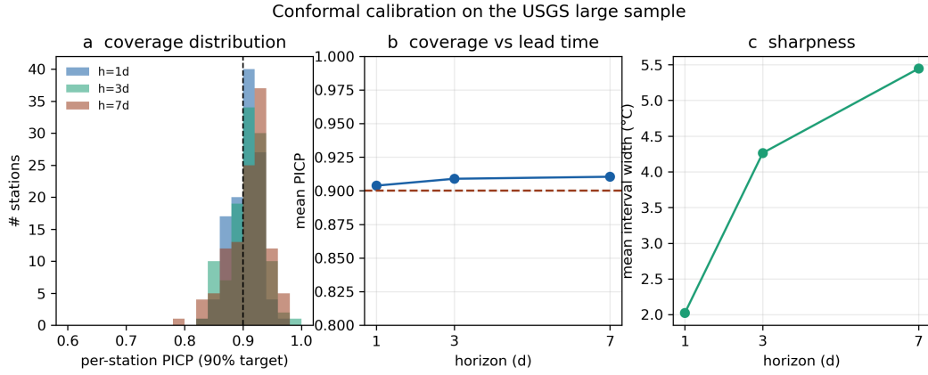
Figure 6. Conformal calibration on n=114 USGS blind-test stations. (a) Per-station coverage (PICP) distribution against the 0.90 target; (b) mean coverage versus lead time; (c) interval sharpness. Coverage is near-nominal and tight across the population (86–96 % of stations within \pm 0.05 of 0.90).
