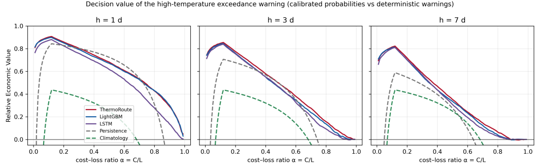
Figure 5. Relative economic value (REV) of the exceedance warning over the full cost-loss ratio grid \alpha (one panel per lead). ThermoRoute’s calibrated warning (solid) dominates LightGBM, the LSTM and the deterministic persistence warning (dashed) across the operational cheap-protection range; the deterministic persistence warning becomes competitive only at high \alpha .
