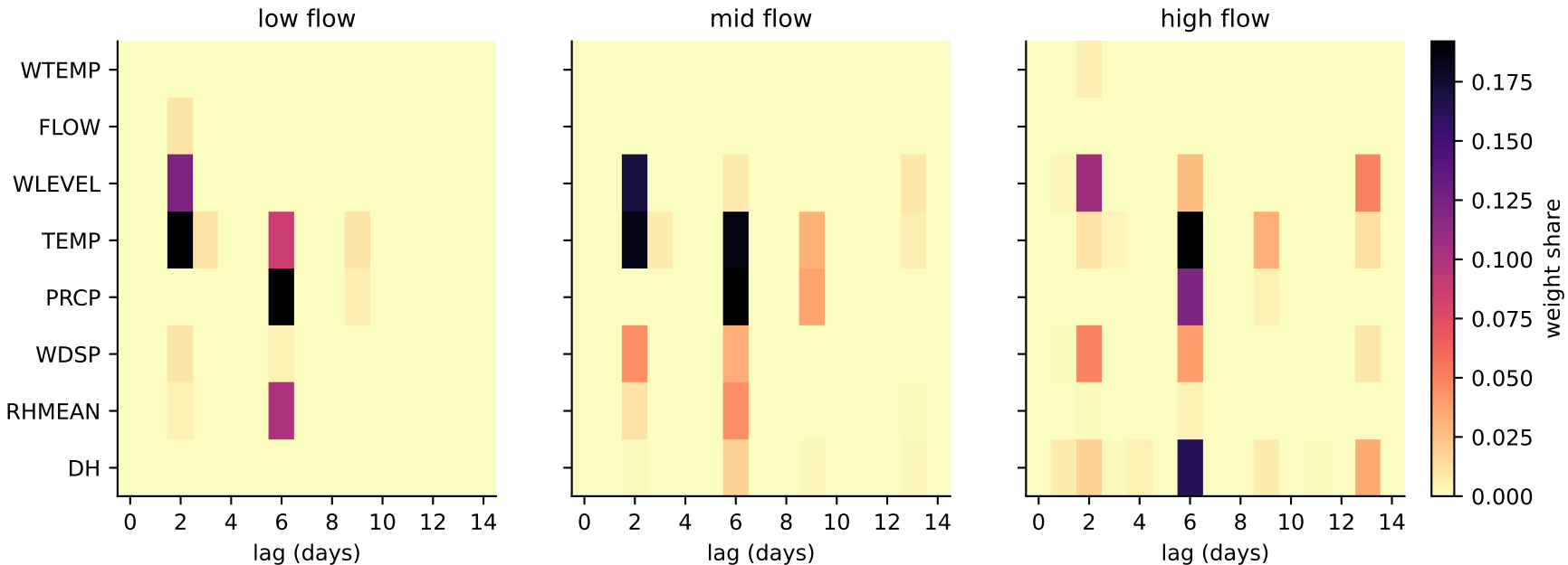
Router lag importance by flow regime (h = 3 d)
