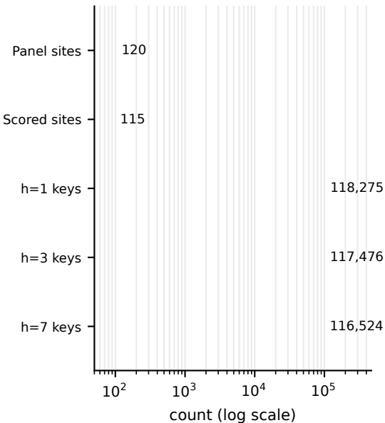
figS6 · missingness and attrition on the held-out 2021-2023 panel
