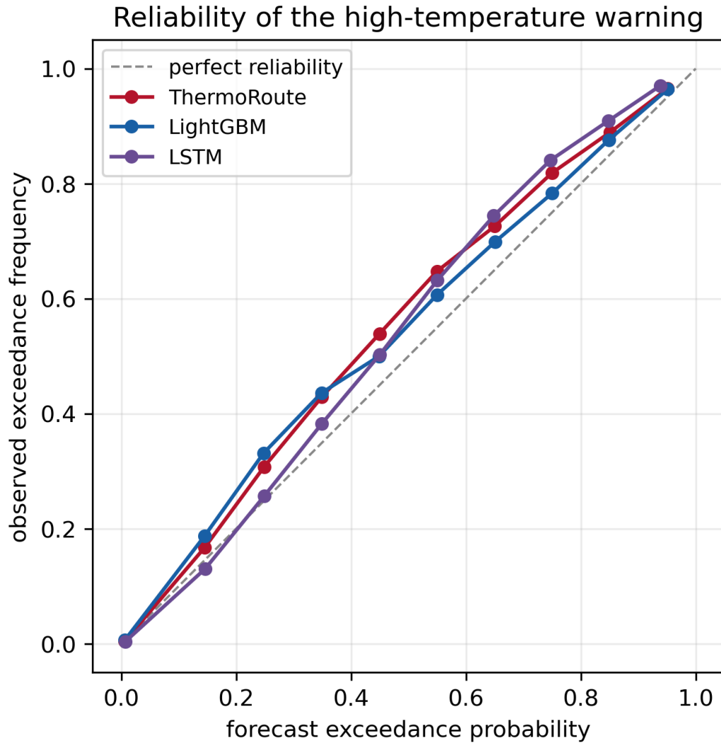
Figure 4. Reliability of the high-temperature exceedance warning (all leads pooled). Forecast probability versus observed exceedance frequency; ThermoRoute’s calibrated warning tracks the diagonal most closely, ahead of the LightGBM and LSTM.
