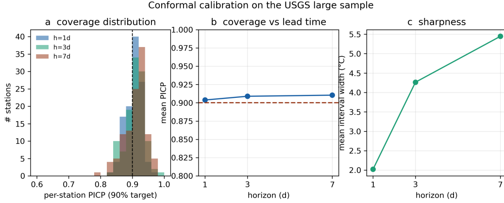
Figure 5. Conformal calibration on n=114 USGS blind-test stations. (a) Per-station coverage (PICP) distribution against the 0.90 target; (b) mean coverage versus lead time; (c) interval sharpness. Coverage is near-nominal and tight across the population (86–96 % of stations within \pm 0.05 of 0.90).
