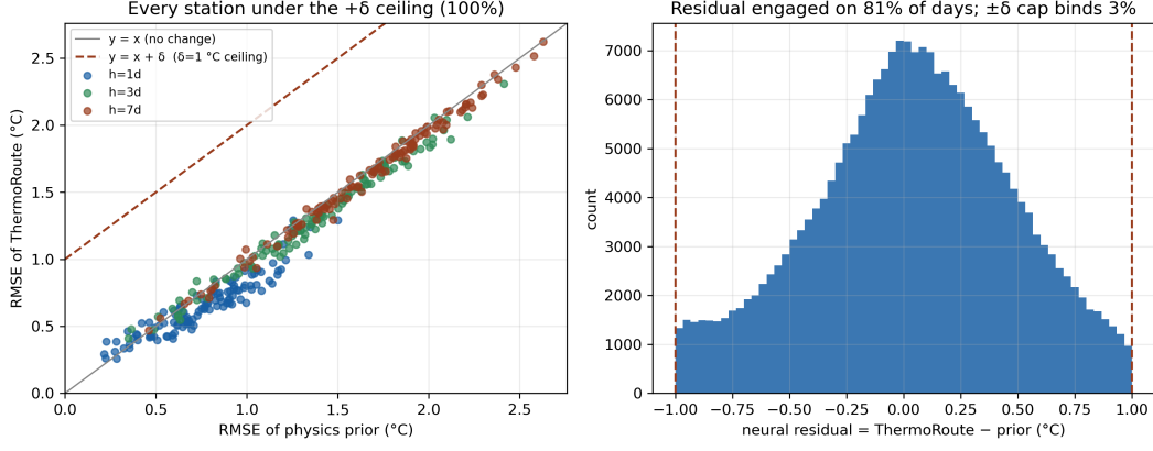
Figure 3. Proposition 1 verified on the blind test. (a) Per-station RMSE of ThermoRoute versus its internal physics prior; every point lies under the y = x + \delta ceiling ( \delta = 1 °C). (b) Distribution of the bounded neural residual: engaged on 81 % of days, but the \pm\delta cap binds on only 3 % — a hard floor the working residual rarely reaches.
