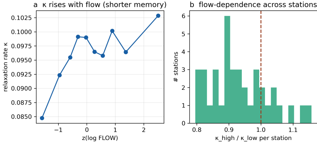
Figure 4: Figure 4. Dynamic relaxation rate \kappa on the 40 USGS stations. (a) \kappa binned by standardised log-flow (pooled); (b) per-station ratio \kappa(\text{high flow})/\kappa(\text{low flow}) . The flow dependence seen on the three reservoir stations does not generalise — \kappa rises with flow at only 18 % of stations (median ratio 0.92) — so we retract the flow-dependent thermal-memory claim.
