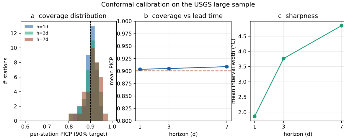
Figure 3: Figure 3. Conformal calibration on the 40 USGS stations. (a) Per-station coverage (PICP) distribution against the 0.90 target; (b) mean coverage versus lead time; (c) interval sharpness. Coverage is near-nominal and tight across the population (89–97 % of stations within \pm 0.05 of 0.90).
