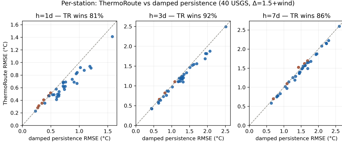
Figure 2: Figure 2. Per-station blind-test RMSE on the 40 USGS stations: ThermoRoute versus damped persistence at 1, 3 and 7 days. Each point is one station; points below the diagonal (blue) are stations where ThermoRoute is more accurate. ThermoRoute wins 81–92 % of stations.
