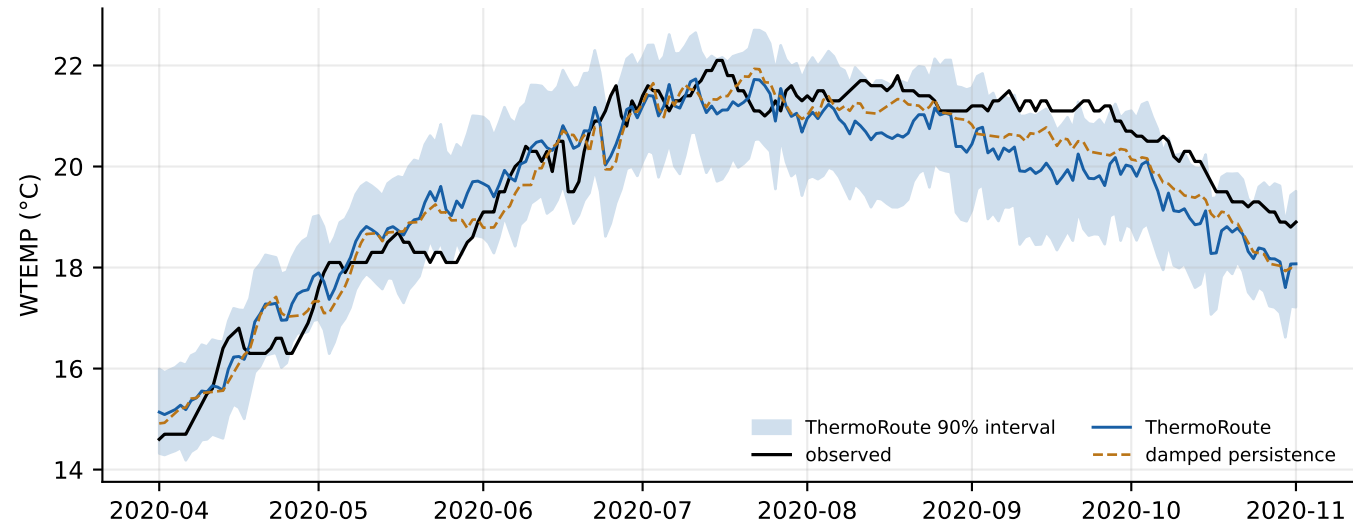
p3, 7-day-ahead blind-test forecast (2020 warm season)
