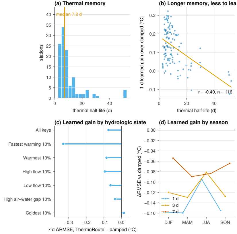
Figure 6. Hydrologic conditions governing incremental skill.
