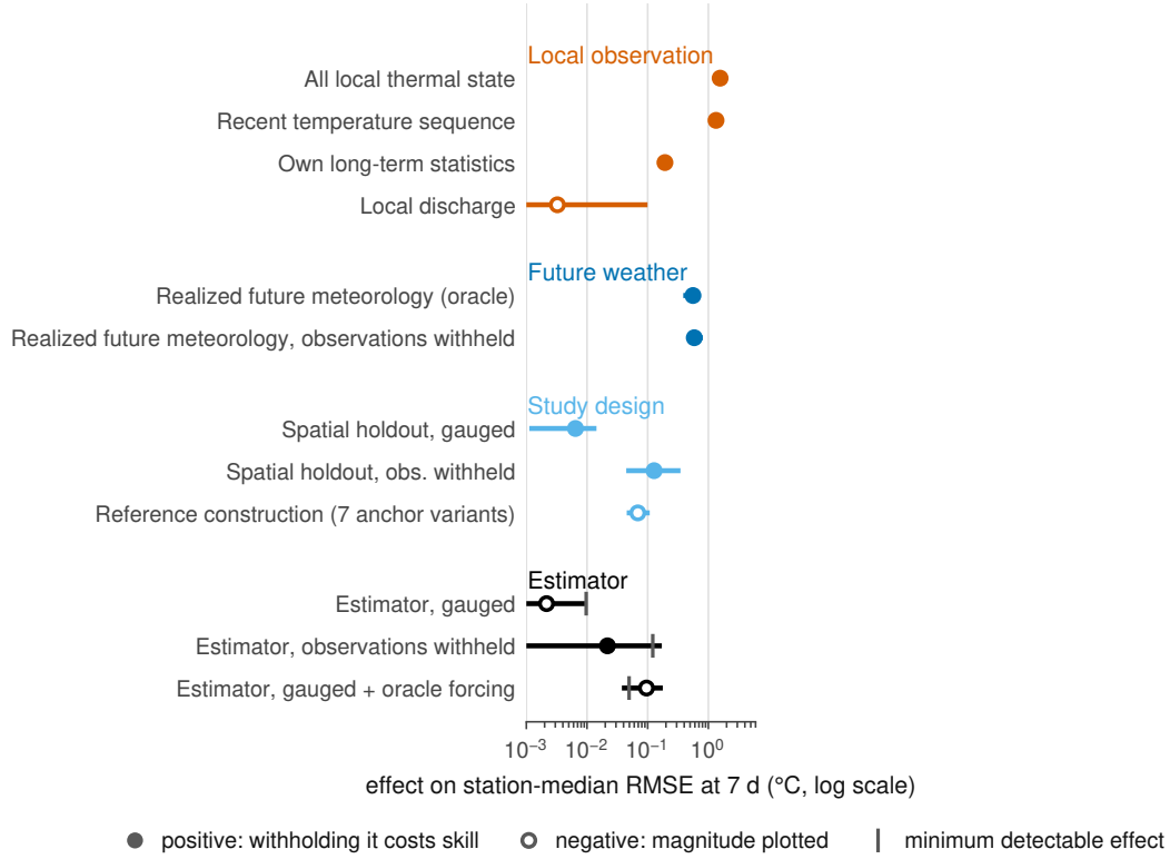
Figure 4. What each axis of the study is worth, at seven days. Station-first paired effects in °C on a log axis, damped-residual tree throughout; open markers are negative effects plotted at their magnitude, and the tick marks the minimum detectable effect where one is defined. Local observation, future weather, study design and the estimator span three orders of magnitude. The axes are separate conditional designs and are compared, never summed. Every row is post-outcome and descriptive except the last, and every bar is a cluster-bootstrap interval except the last: reference construction is the range across the seven predeclared anchor variants of Section 4.1 — a spread over specifications, not a sampling interval. It is on this axis because every other row is conditional on one anchor while the anchor is itself a fitted object, and it says how much of the figure is a property of the reference rather than of the river.
