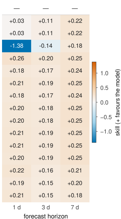
(b) Skill vs persistence
