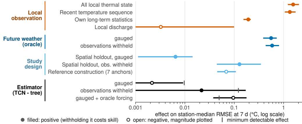
Figure 4. What each axis of the study is worth, at seven days. Station-first paired effects in ^{\circ}\text{C} on a log axis, damped-residual tree throughout; open markers are negative effects plotted at their magnitude, bars that reach the 0.001 floor are intervals spanning zero, and the tick marks the minimum detectable effect where one is defined. Within Future weather (oracle) and Estimator the row label gives only what distinguishes it — “gauged” is L0 and “observations withheld” is L2 — and the bracket carries the rest, so Estimator rows are the plain causal network minus the tree. Local observation, future weather, study design and the estimator span three orders of magnitude on one continuous axis; the axes are separate conditional designs and are compared, never summed. Every row is post-outcome and descriptive except reference construction , whose bar is also the one interval that is not a cluster bootstrap: it is the range across the seven predeclared anchor variants of Section 4.1, a spread over specifications. It is on this axis because every other row is conditional on one anchor while the anchor is itself a fitted object, and it says how much of the figure is a property of the reference rather than of the river.
