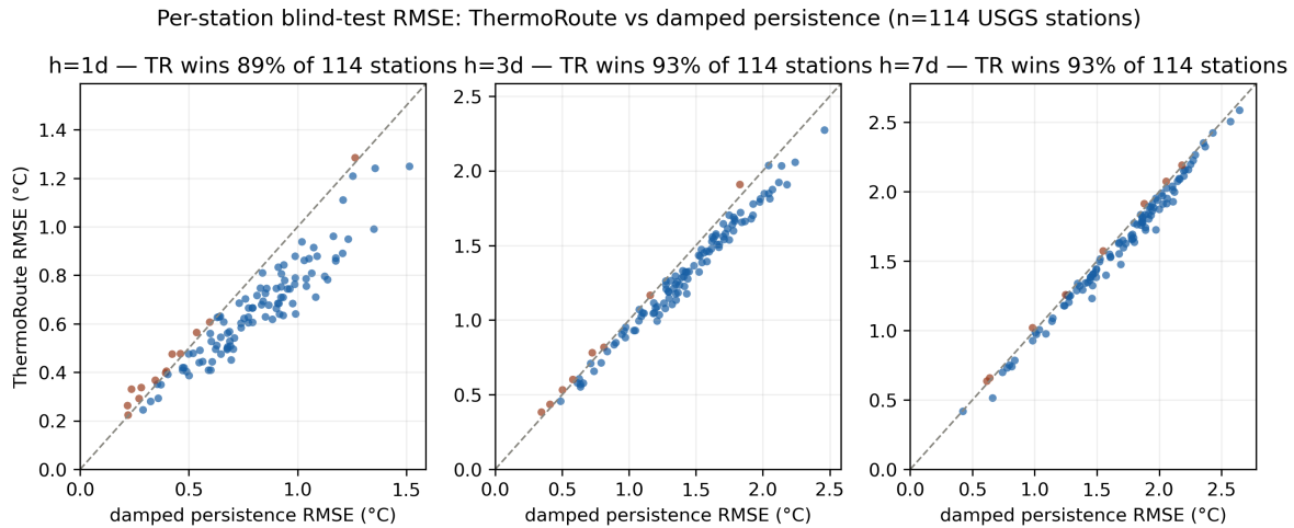
Figure 2: Figure 2. Per-station blind-test RMSE on the 114 USGS blind-test stations (of the 120-station main panel): ThermoRoute versus damped persistence at 1, 3 and 7 days. Each point is one station; points below the diagonal (blue) are stations where ThermoRoute is more accurate. ThermoRoute wins 89–93 % of stations.
