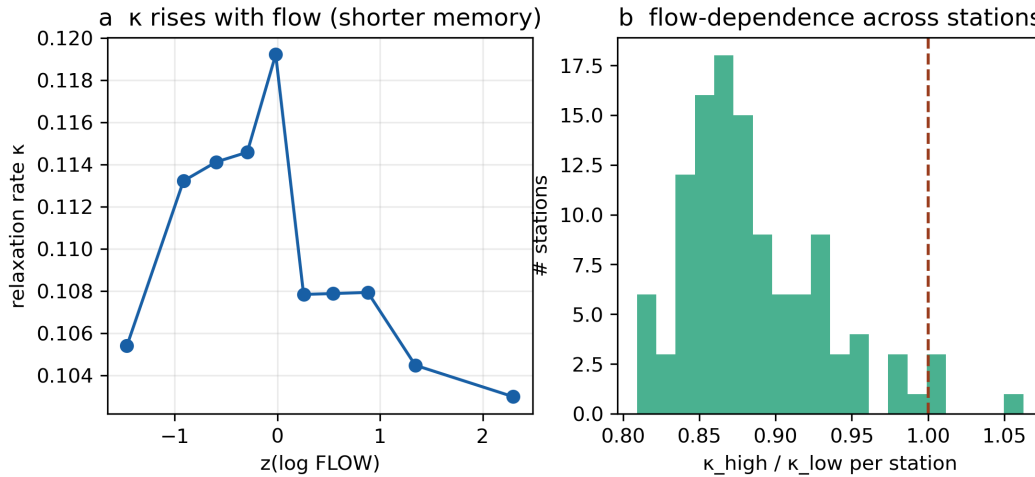
Figure 4: Figure 4. Dynamic relaxation rate \kappa on the 120-station USGS panel. (a) \kappa binned by standardised log-flow (pooled); (b) per-station ratio \kappa(\text{high flow})/\kappa(\text{low flow}) . The flow dependence seen on the three reservoir stations does not generalise — \kappa rises with flow at only 2 % of stations on the 120-station panel (and 24 % on the 40-station intermediate that we report for comparison), median ratio 0.87 — so we retract the flow-dependent thermal-memory claim.
