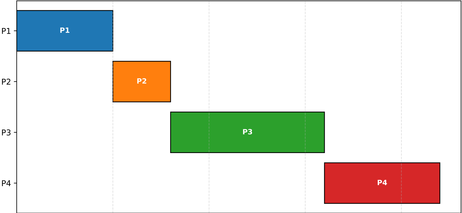
FCFS - Gantt Chart
