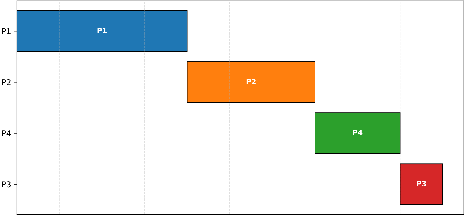
Priority (Non-Preemptive) - Gantt Chart
