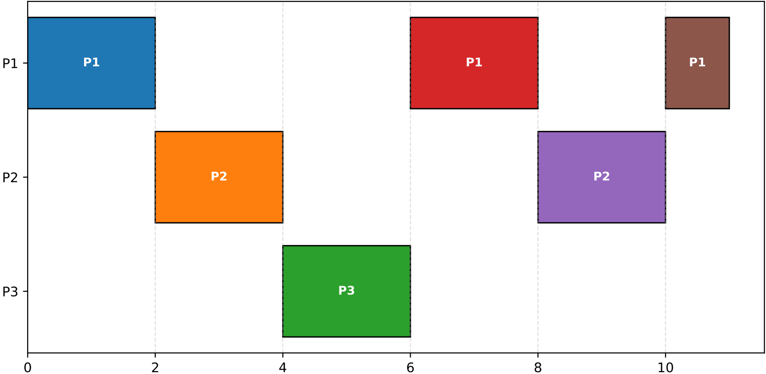
Round Robin - Gantt Chart
