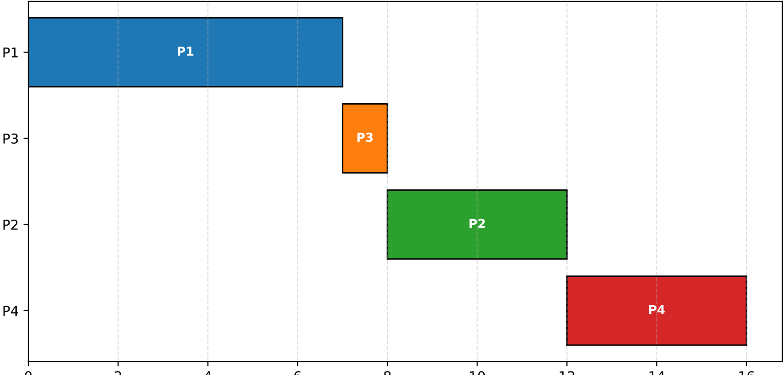
SJF (Non-Preemptive) - Gantt Chart
