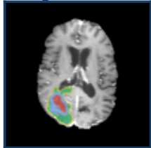
Segmentation
