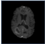
T1ce
