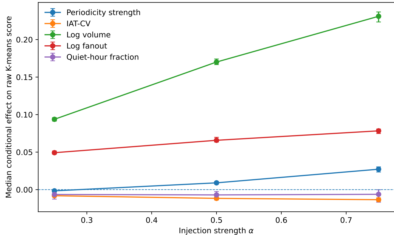
K-means score sensitivity to each injected CORE5 feature
