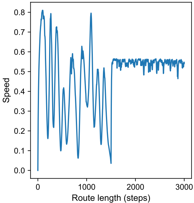
Speed
