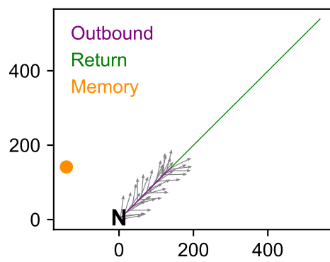
Bounded random
