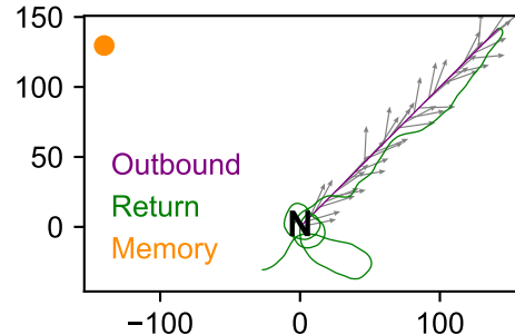
Bounded random
