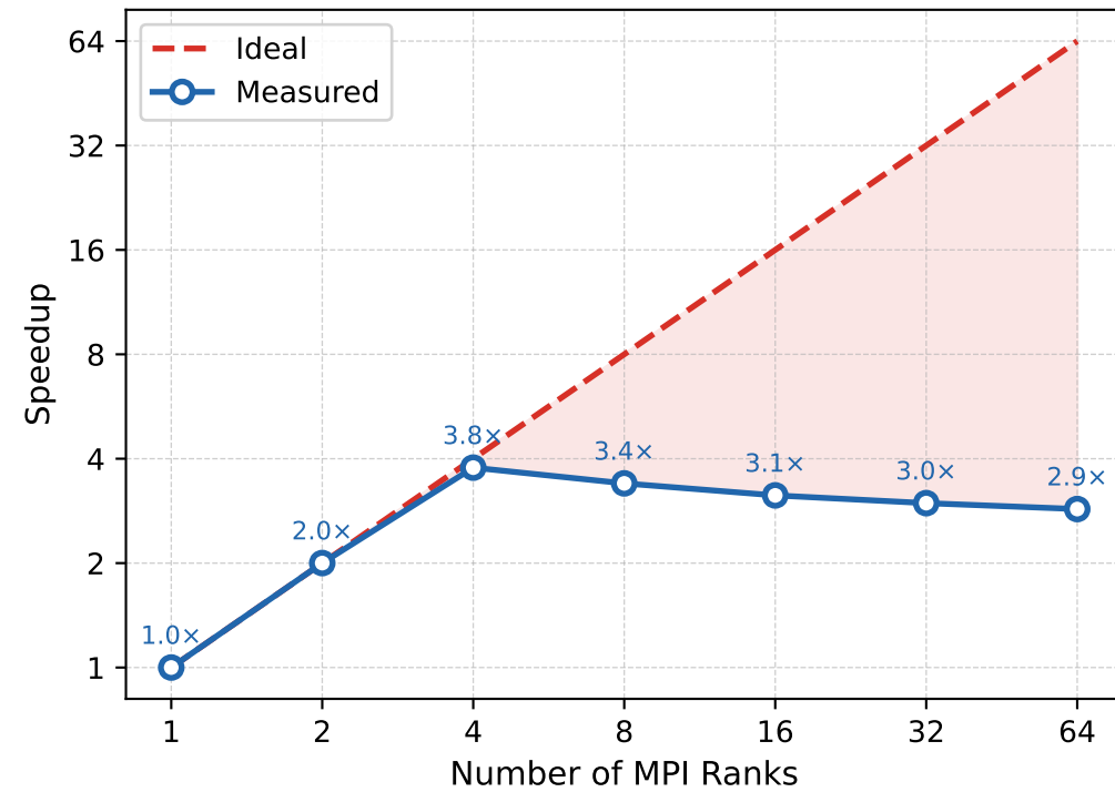
(b) Speedup (relative to 1 rank)
