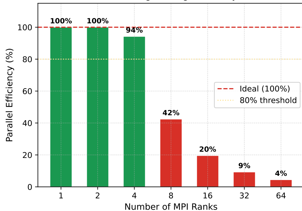
(c) Strong Scaling Efficiency
