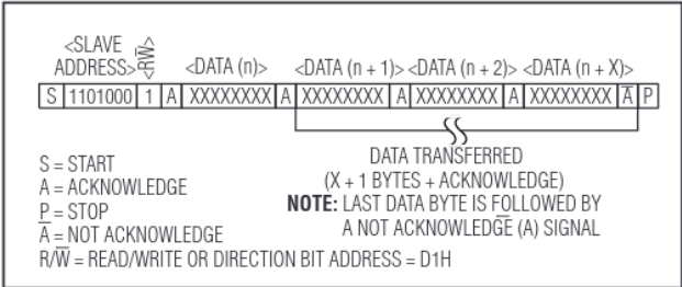
Figure 4. Slave Transmitter Mode (Read Mode)
