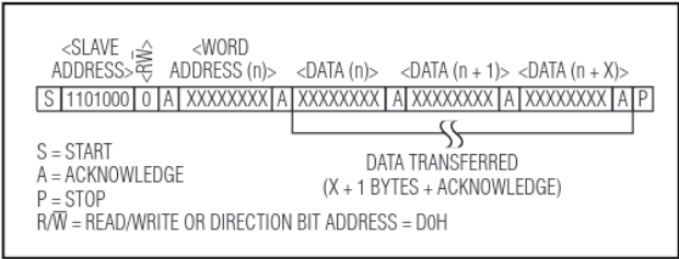
Figure 3. Slave Receiver Mode (Write Mode)
