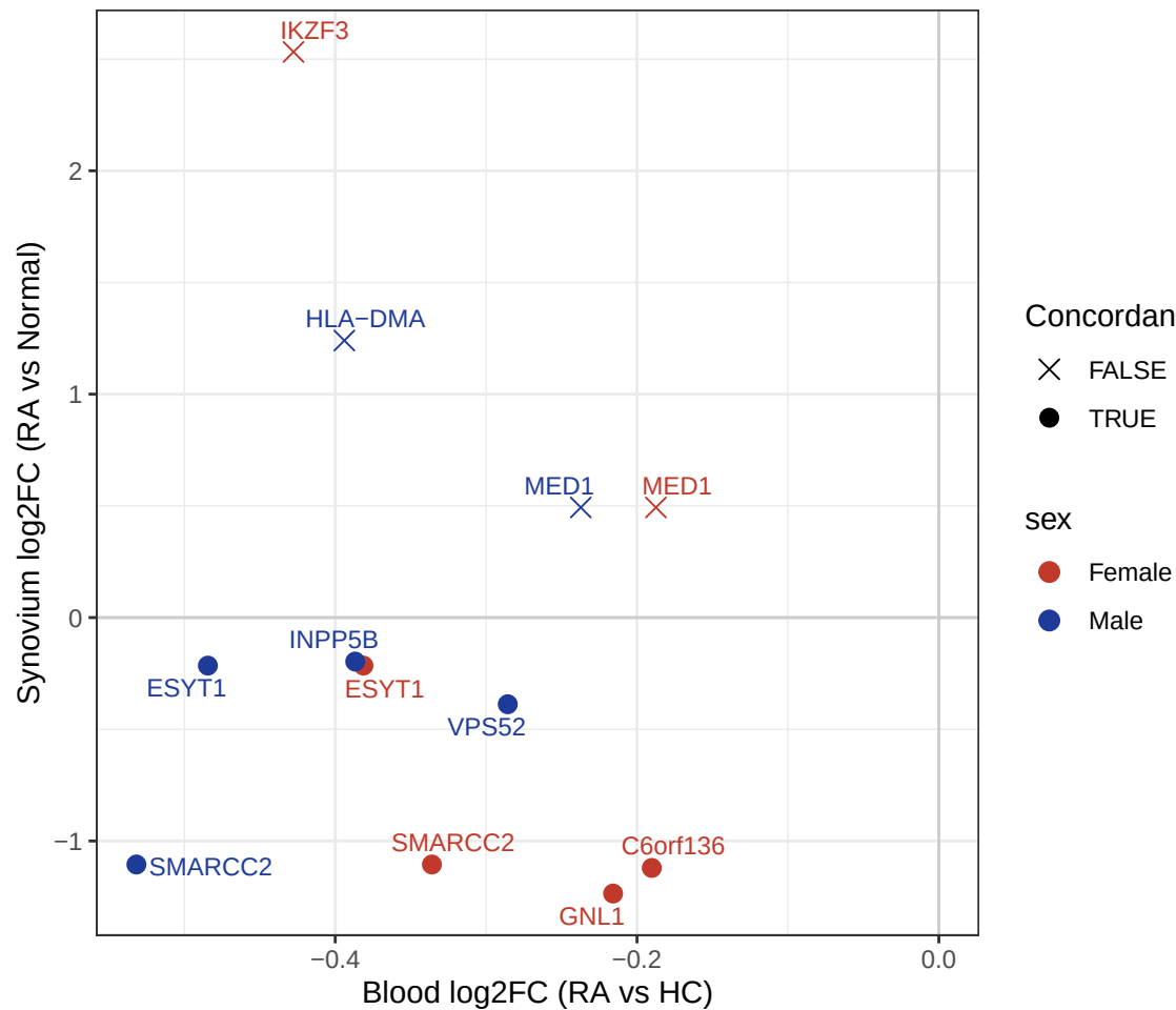
A Blood vs synovium concordance
