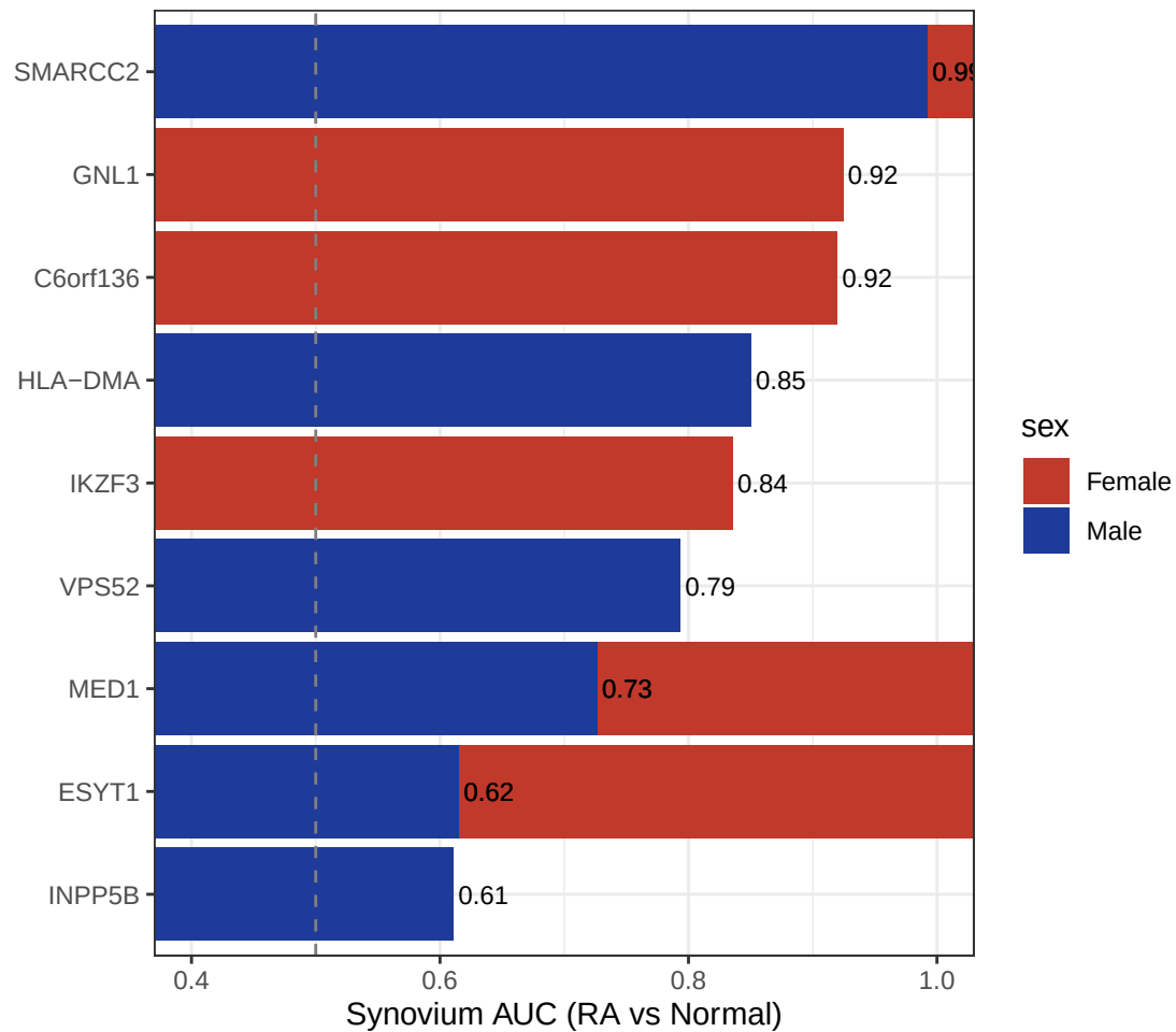
B Per-gene synovium discrimination
