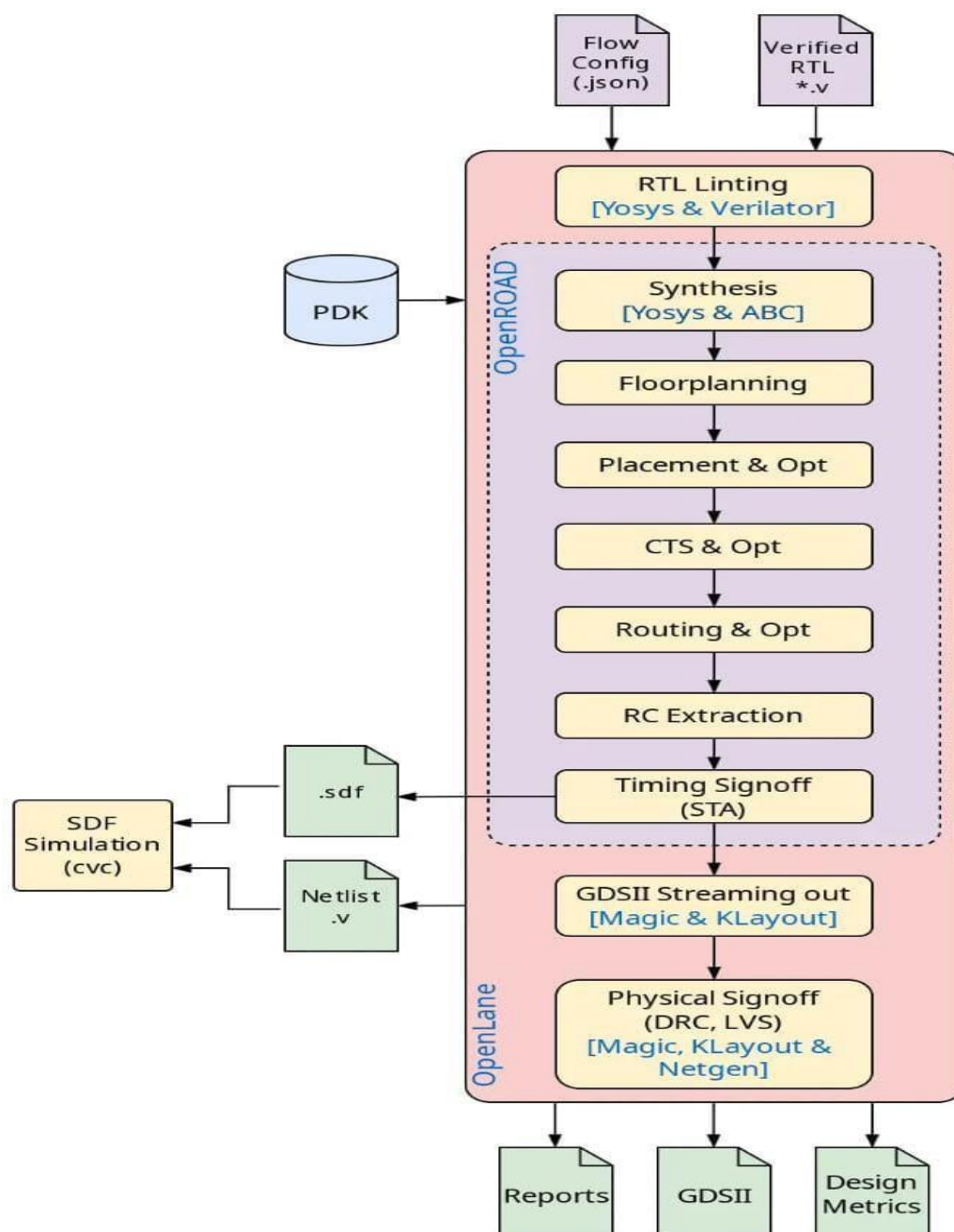
Fig4.1: Flowchart of the OpenLane SKY130A physical design process from RTL input final GDSII output.
