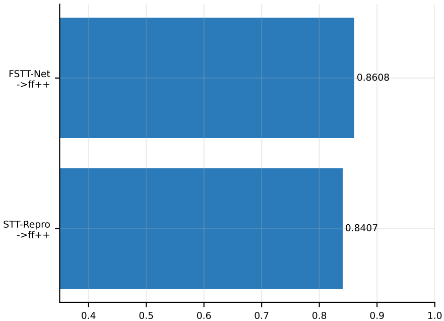
Cross-dataset frame AUC (trained on celebdf)
