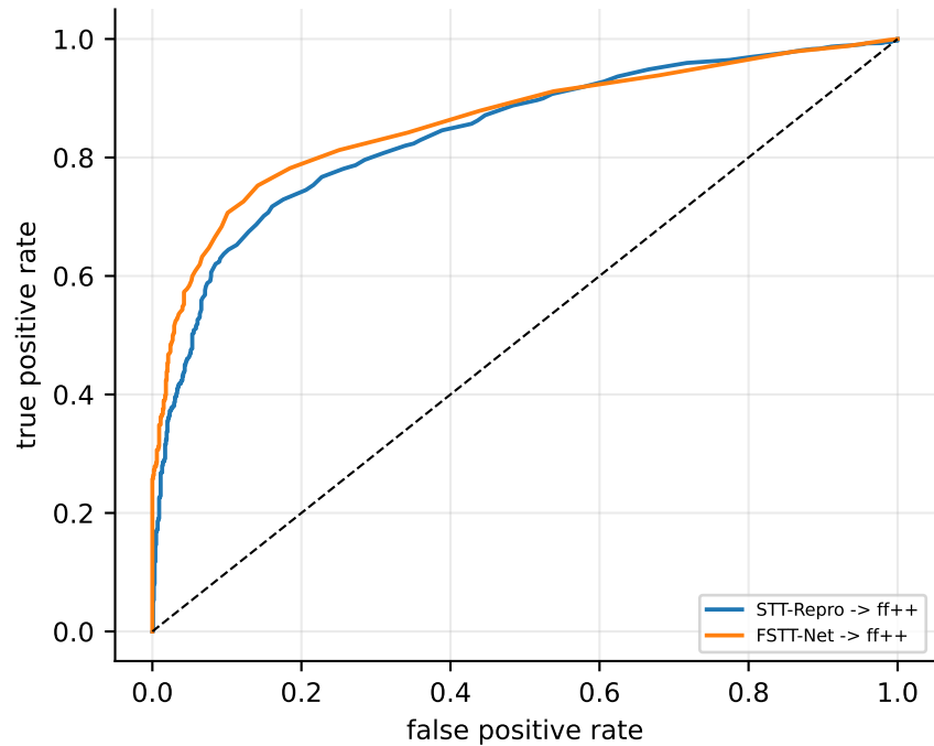
Cross-dataset ROC
