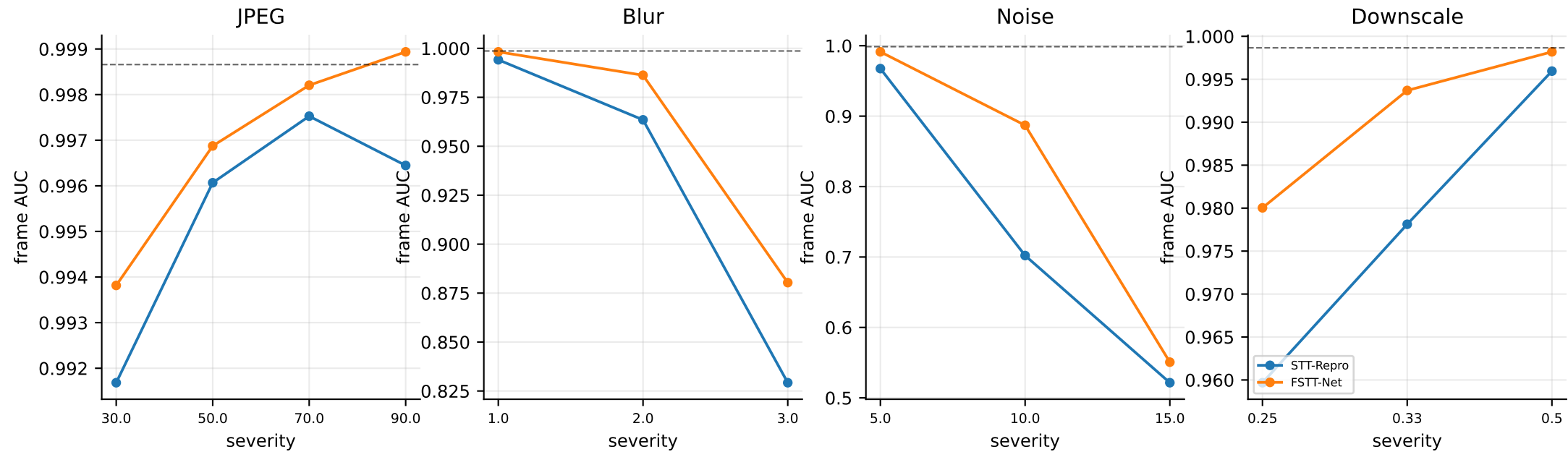
Robustness to real-world degradation (dashed = clean mean)
