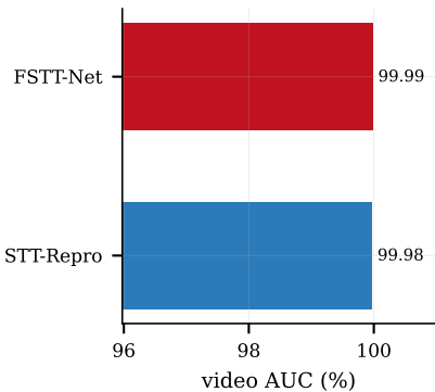
(a) Benchmark
