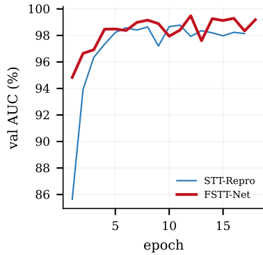
(e) Convergence
