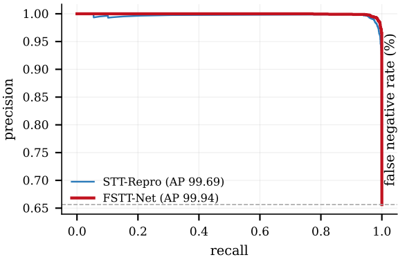
(a) Precision-recall
