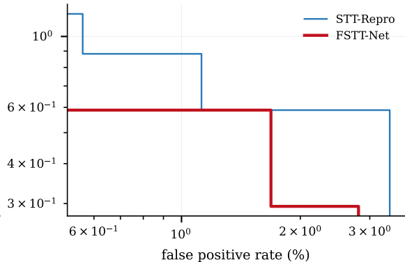
(b) DET, video level
