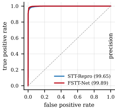
(a) ROC, frame
