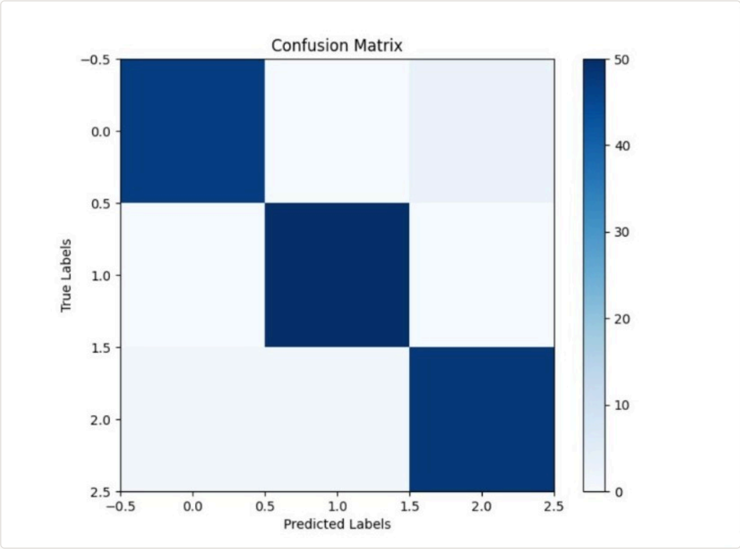
Fig 1: Mathematical matrix confirming a clean 0.97 macro average across food (1.00 recall) and miscellaneous classes.
