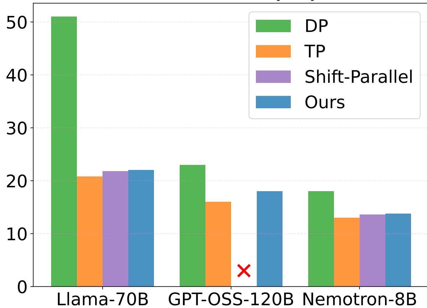
Median TPOT(ms)
