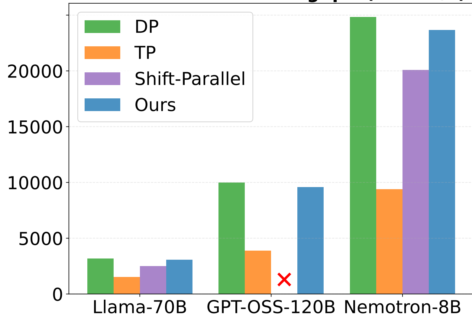
Peak Generation Throughput(tokens/s)
