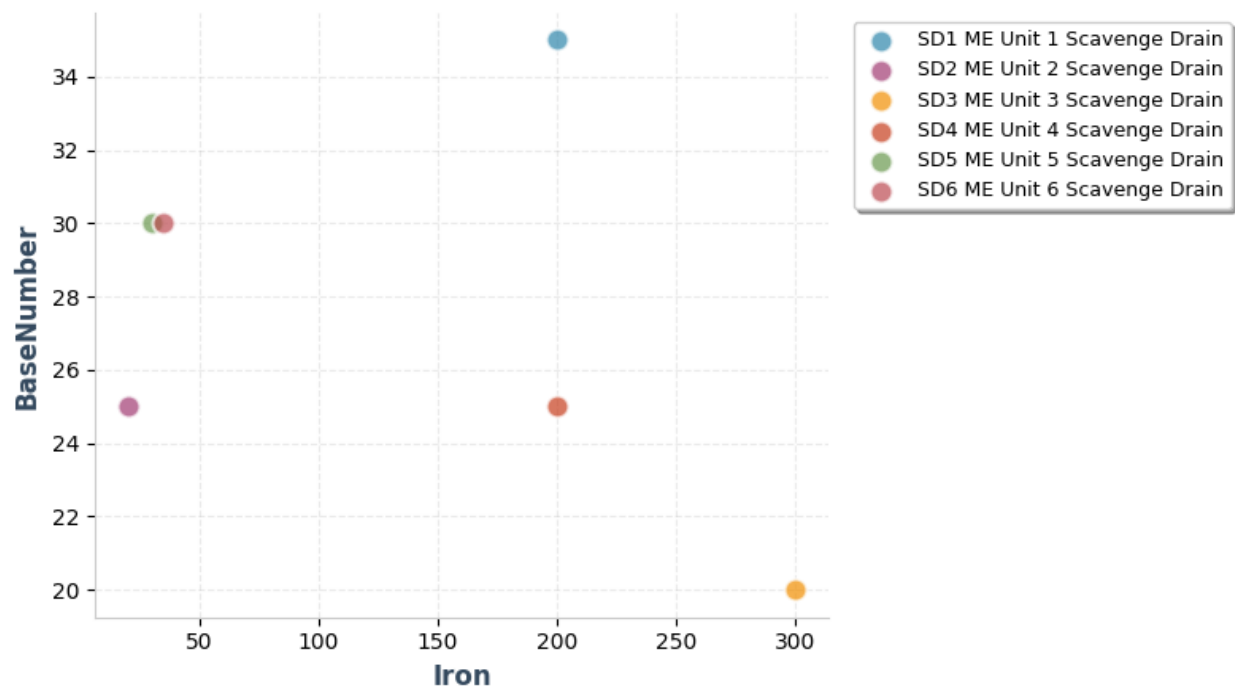
Scavenge Drain - Iron vs Base Number
