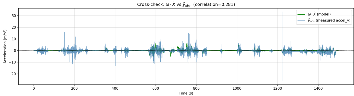
Figure 7: Cross-check: model prediction \omega \dot{X} (green) vs. measured lateral acceleration \ddot{y}_{obs} (blue). Both signals are near zero except at turns. Pearson correlation is +0.28, indicating qualitative agreement but significant quantitative discrepancy.
