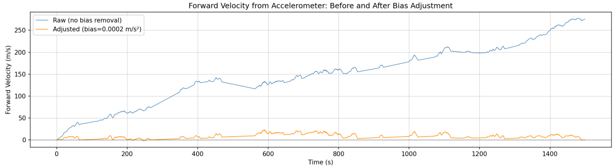
Figure 5: Forward velocity from accelerometer before (raw, blue) and after (adjusted, orange) gravity and bias correction. The raw signal drifts to +250 m/s due to the 0.549 m/s 2 gravity leak. After correction the velocity stays near zero but still drifts slowly due to unavoidable integration error.
