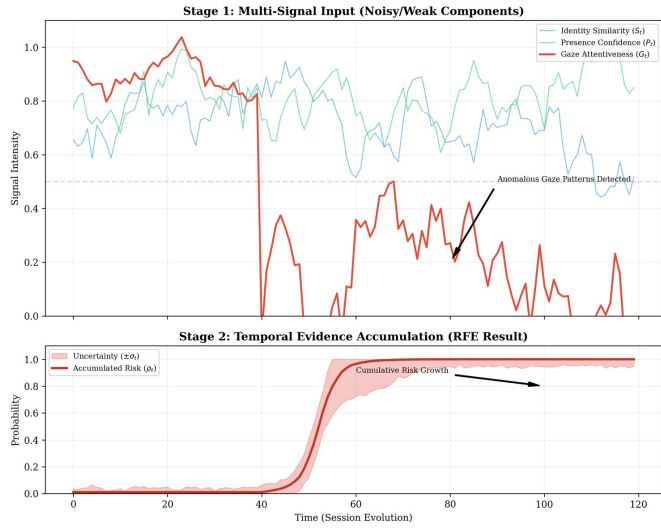
Fig. 9. Evidence accumulation. Weak, noisy signals are integrated into a stable risk trajectory, suppressing frame-level uncertainty.
