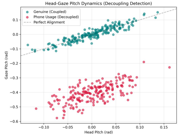
Fig. 10. Pose-gaze decoupling. Genuine behavior (coupled) maintains strong pitch correlation, while phone usage and side-monitor glancing create distribution shifts captured by HGDM.
