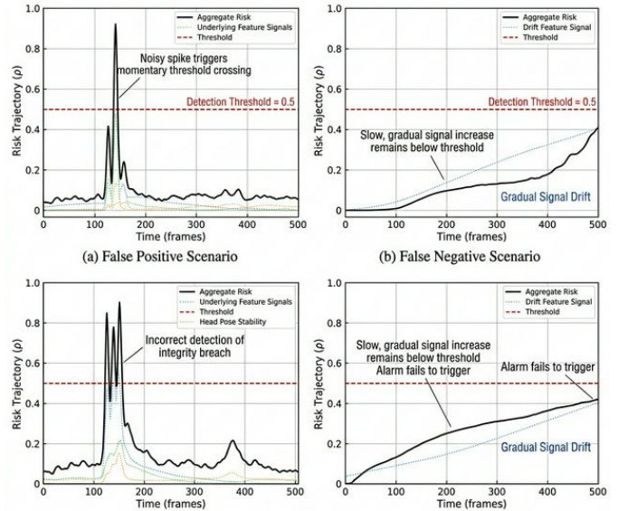
Figure 4: Analysis of typical failure modes in online AI proctoring systems: (a) False Positive due to sensor noise spikes, (b) False Negative due to gradual signal drift.
