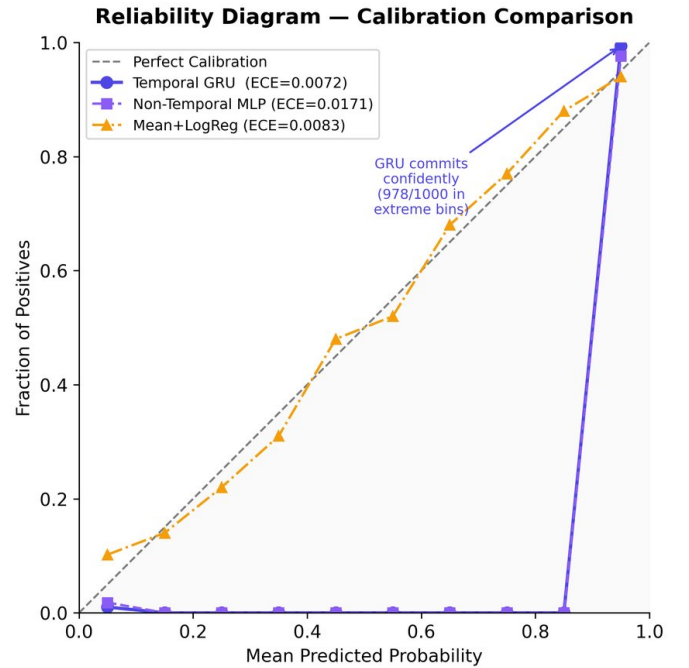
Fig. 7. Reliability diagram. The GRU achieves ECE = 0.0072 with concentrated extreme-bin predictions.
