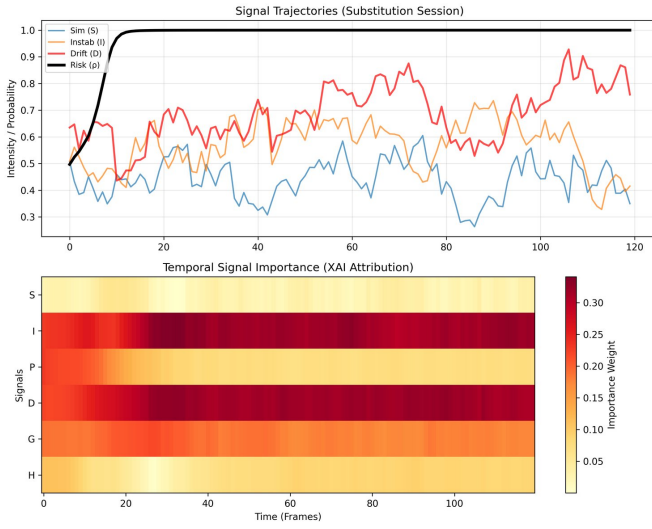
Fig. 11. Temporal signal attribution. Top : signal trajectories during a substitution session. Bottom : attribution heatmap showing signal importance. Drift ( D ) and Instability ( I ) dominate as \rho_t increases.
