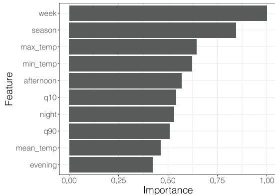
Fig. 8. Aggregate feature importance for EDA \leq 1 .
