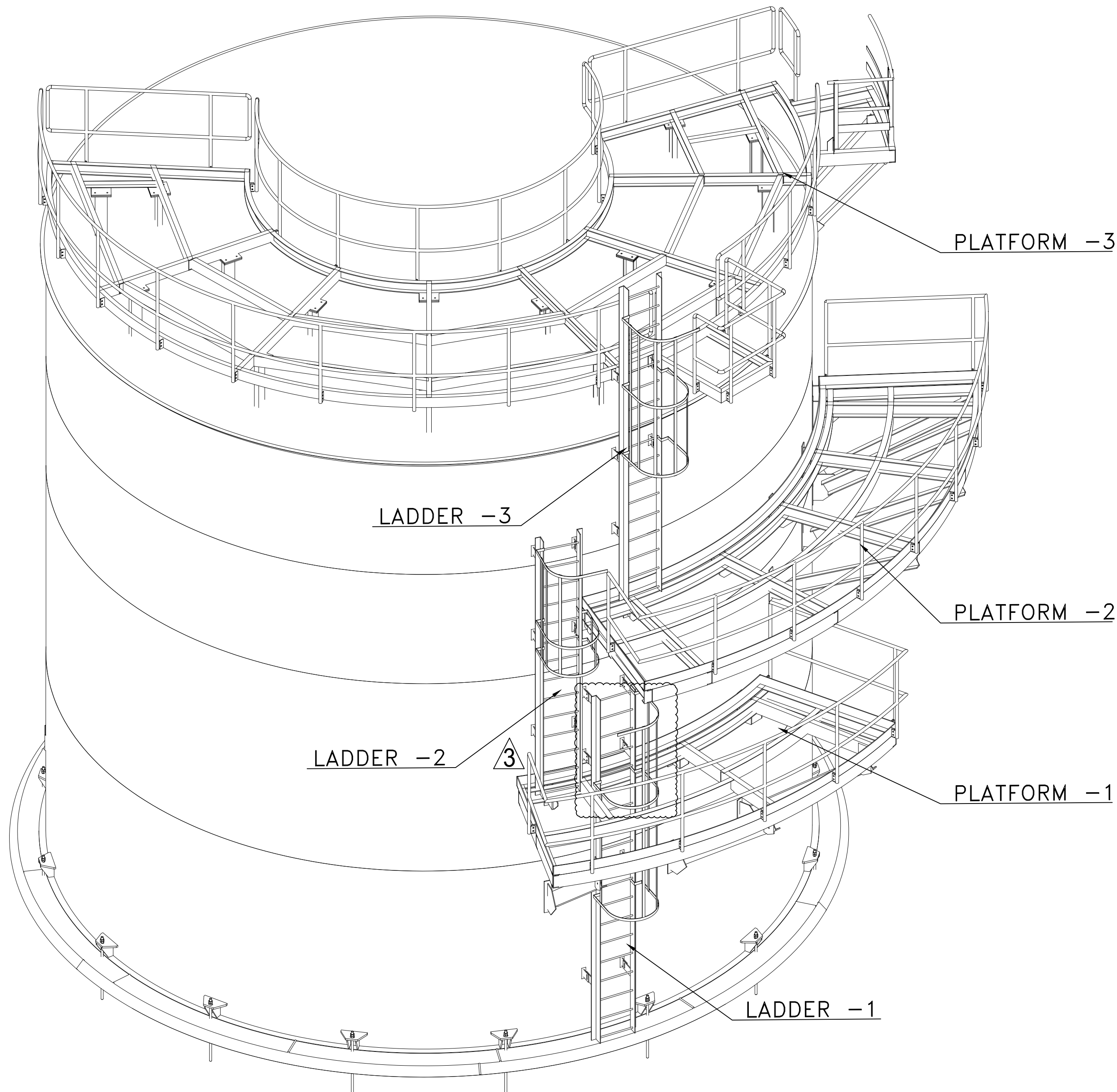
ISOMETRIC VIEW ASSEMBLY DETAILS FOR LADDER CONNECTION
