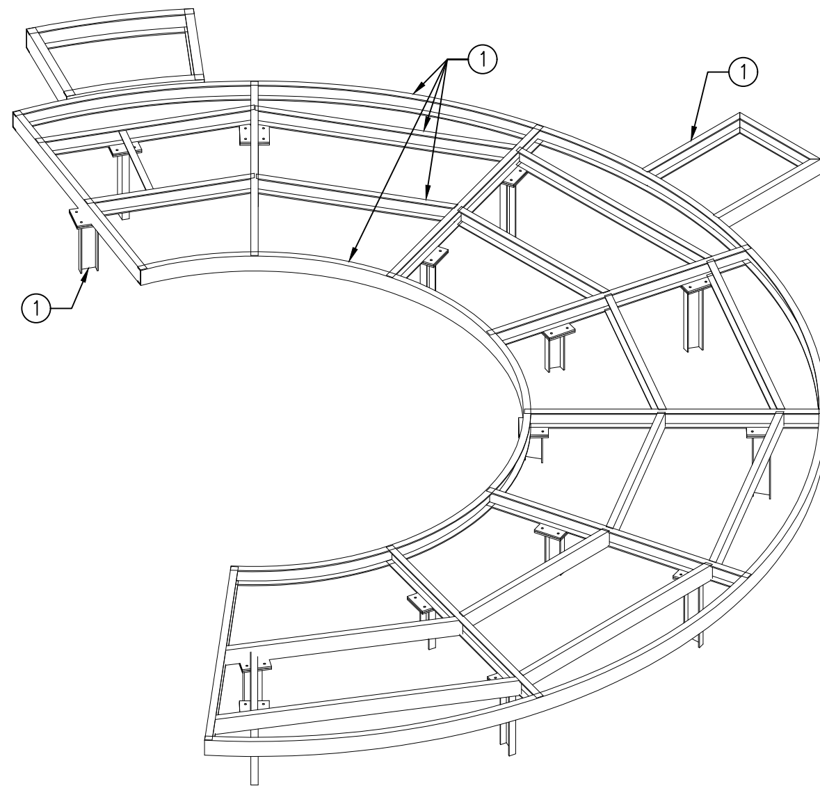
ISOMETRIC VIEW PLATFORM - 3
