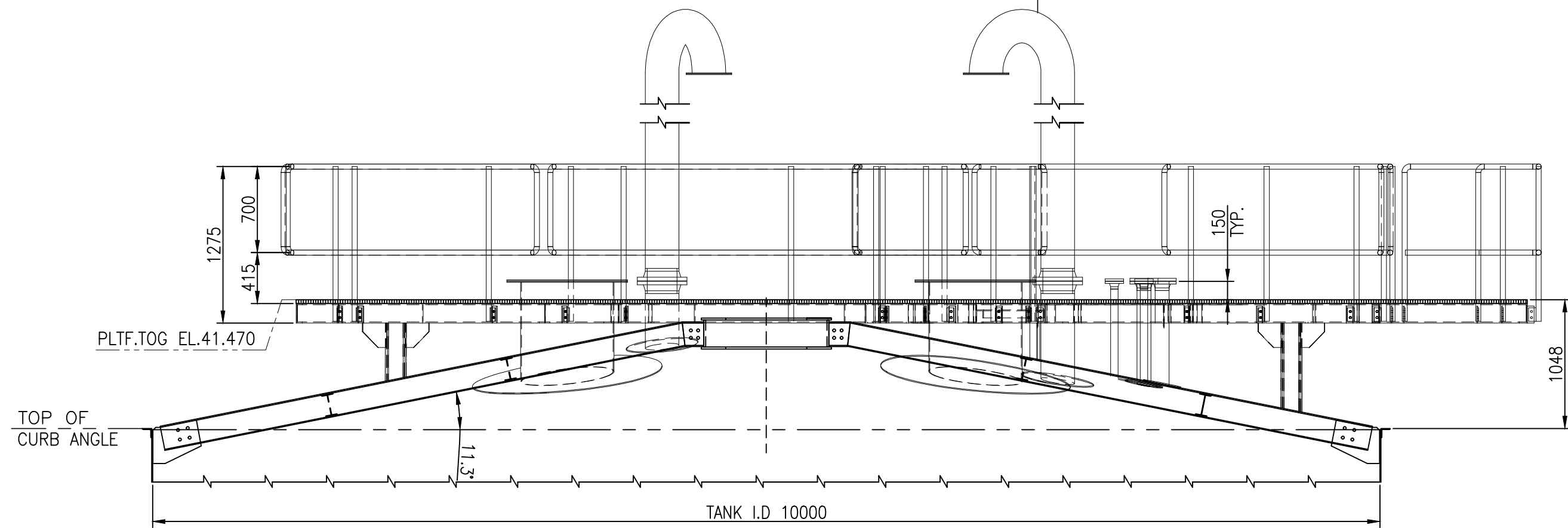
ELEVATION VIEW
