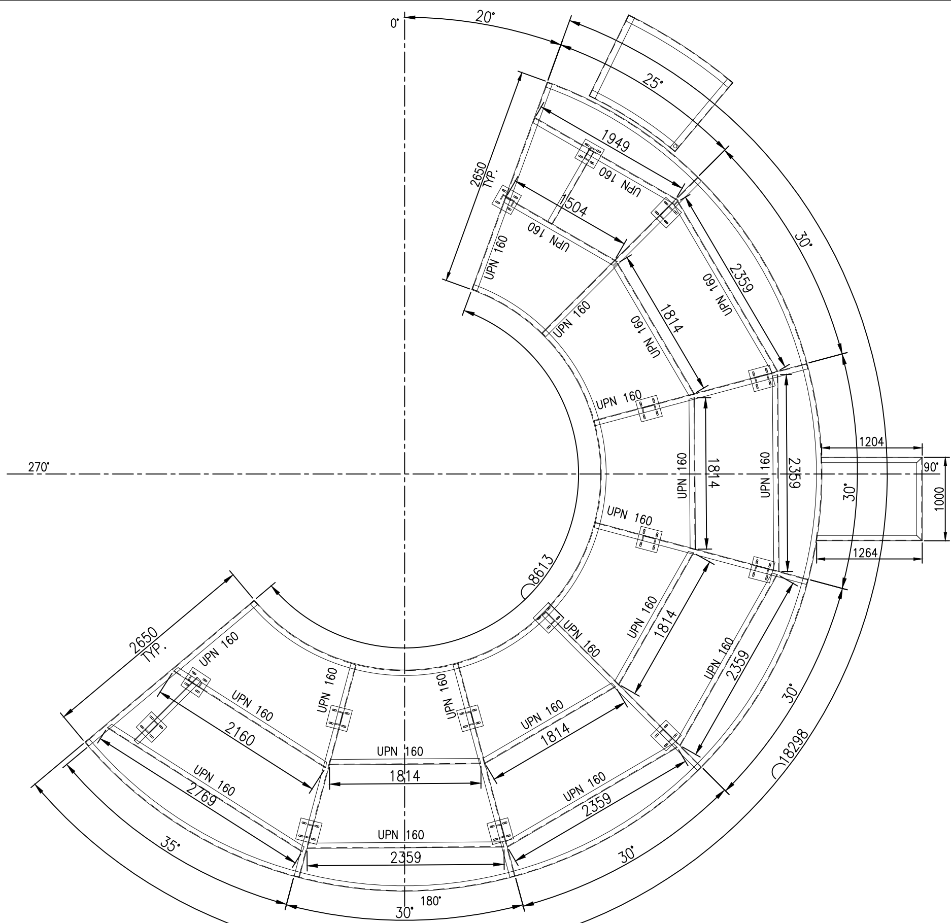
PLAN VIEW PRIMARY & SECONDARY MEMBER DETAILS (PLATFORM-3)
