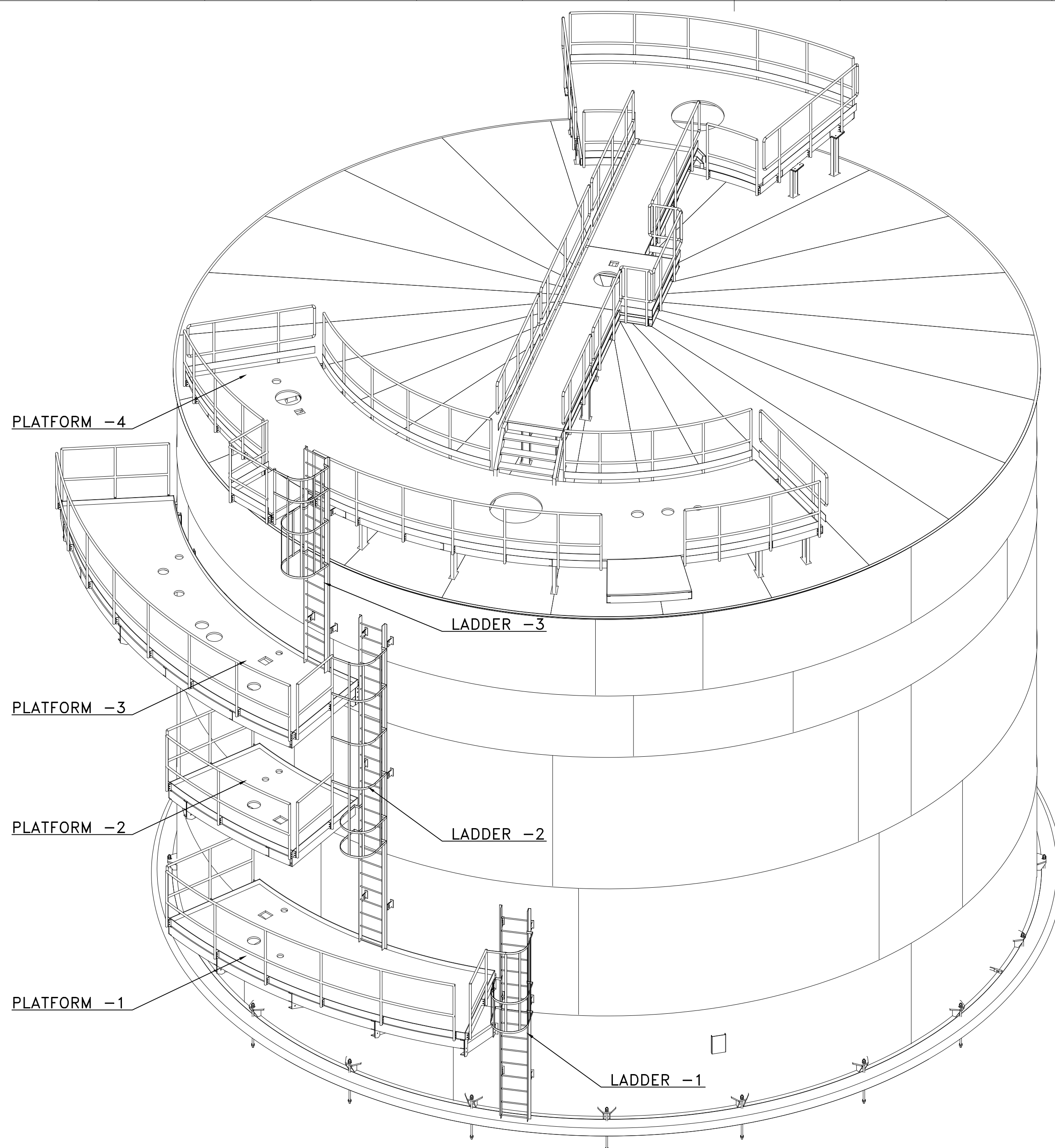
ISOMETRIC VIEW ASSEMBLY DETAILS FOR LADDER CONNECTION
