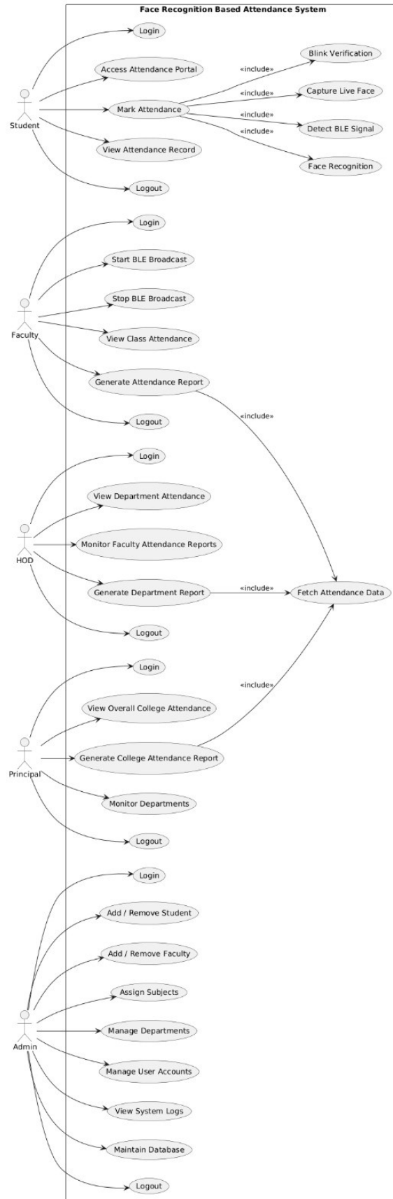
Face Recognition Based Attendance System - Use Case Diagram
