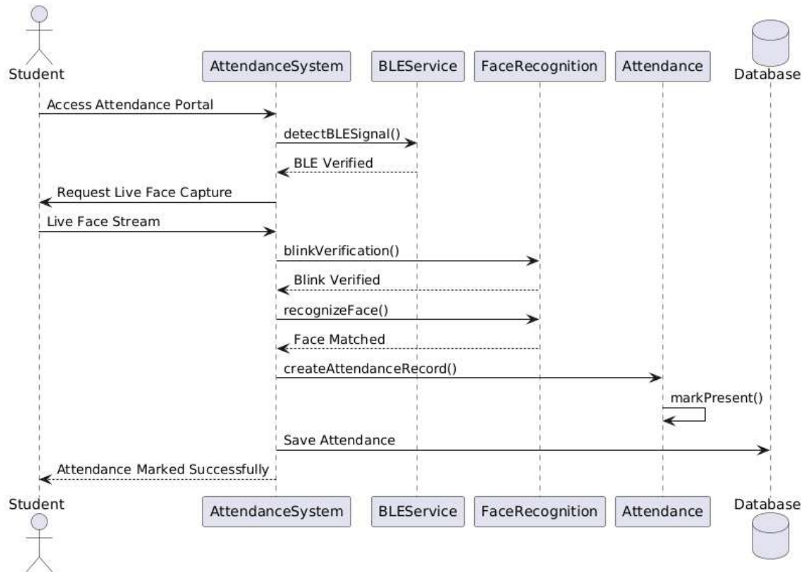
Sequence Diagram - Mark Attendance
