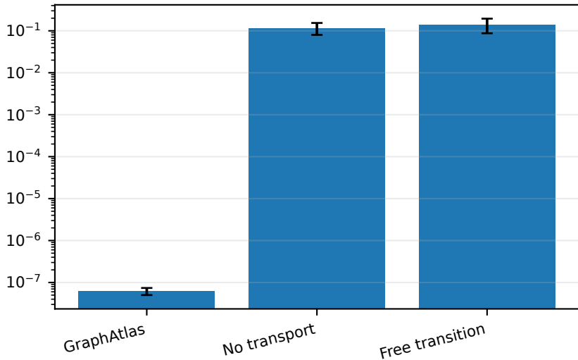
Coordinate reparameterization stability
