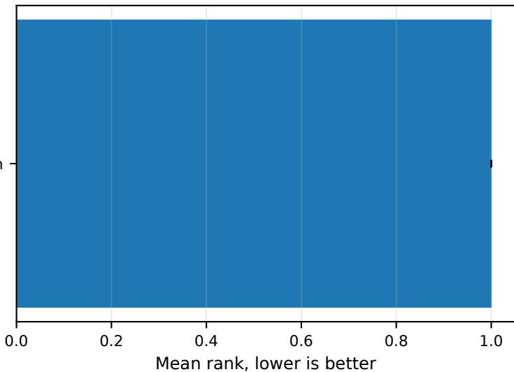
Node Classification
