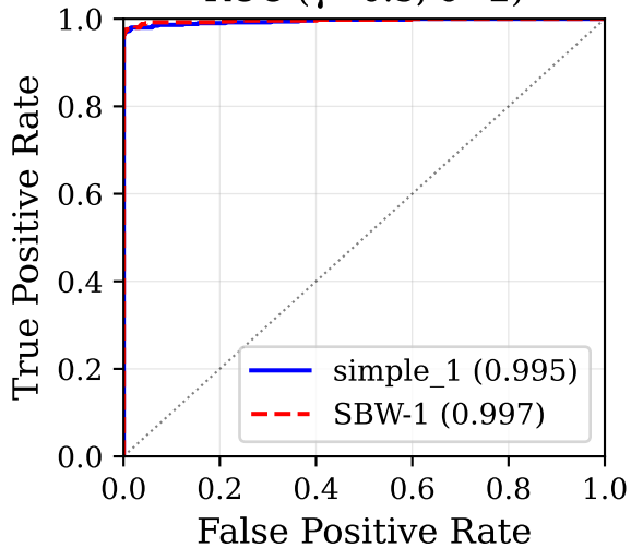
ROC ( \gamma=0.5 , \delta=2 )
