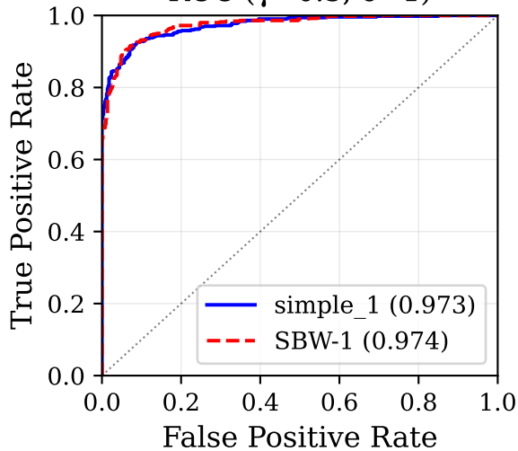
ROC ( \gamma=0.5 , \delta=1 )
