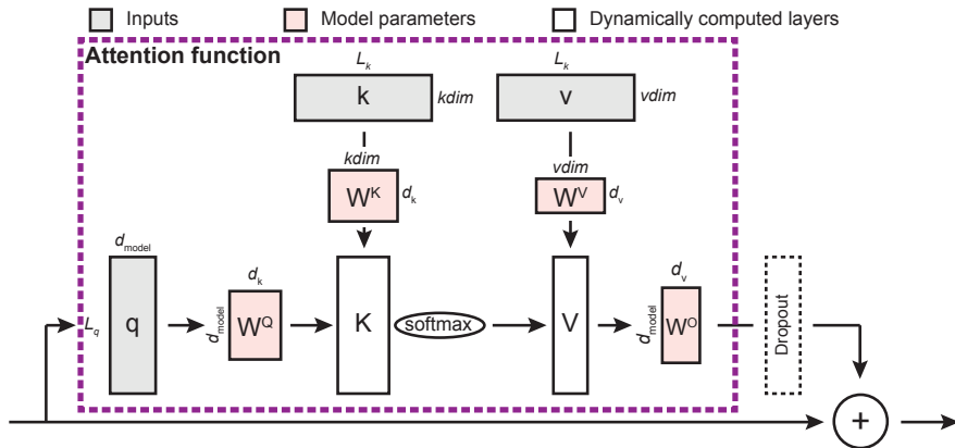
Figure 1: Attention function and the residual stream. This figure visually describes the function discussed in this document. It also shows the residual stream (bottom arrow and the summation \oplus ) and the (optional) dropout layer.
