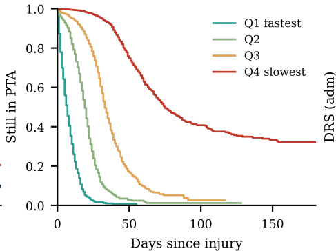
(b) Risk stratification (test)
